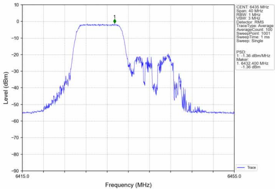
802.11ax(HEW20)_LCH_6435MHz_RU106 / _Ant5_NTNV
