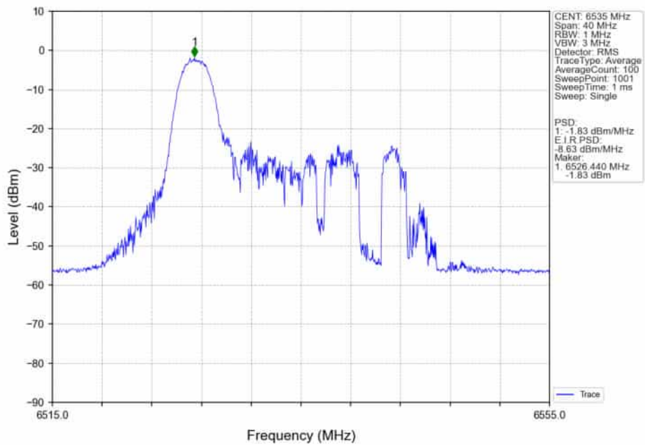
802.11ax(HEW20)_LCH_6535MHz_RU26 / _Ant5_NTNV
