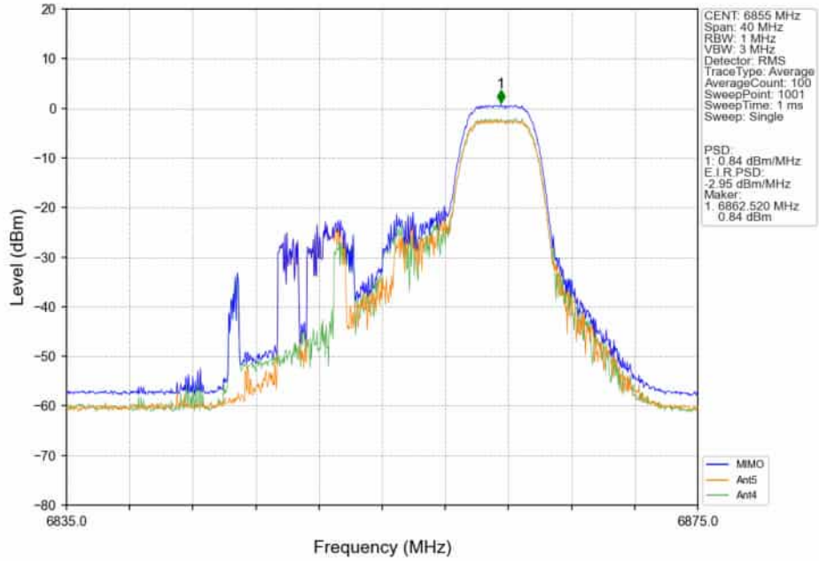
802.11ax(HEW20)_HCH_6855MHz_RU106_/_Ant5_NTNV
