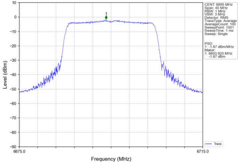
802.11ax(HEW20)_MCH_6695MHz_SU_/_Ant4_NTNV
