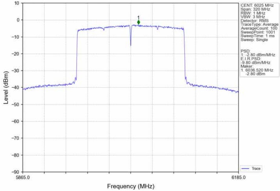
802.11ax(HEW160)_LCH_6025MHz_SU_ / _MIMO_NTNV
