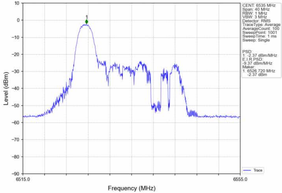
802.11ax(HEW20)_LCH_6535MHz_RU26_/_MIMO_NTNV
