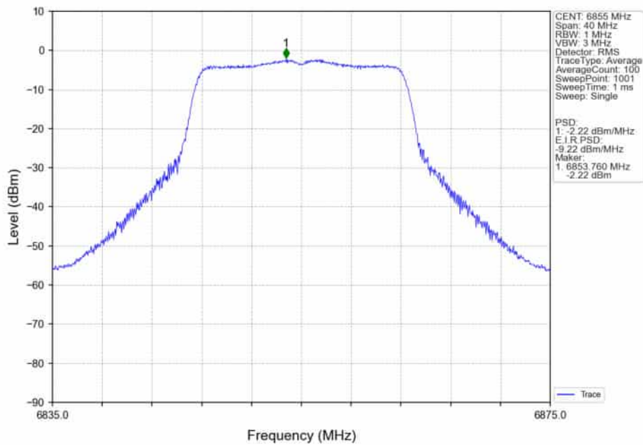
802.11a_HCH_6855MHz_Ant4_NTNV
