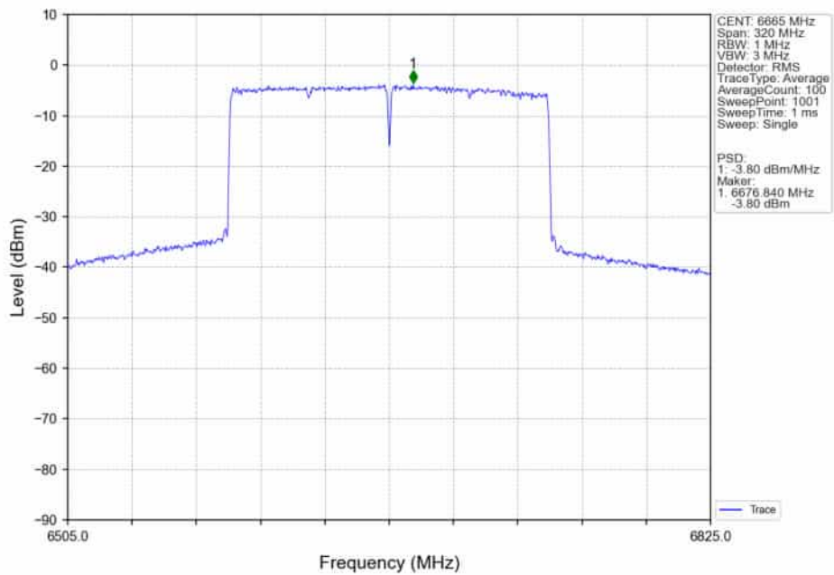
802.11ax(HEW160)_MCH_6665MHz_SU_ / _Ant5_NTNV
