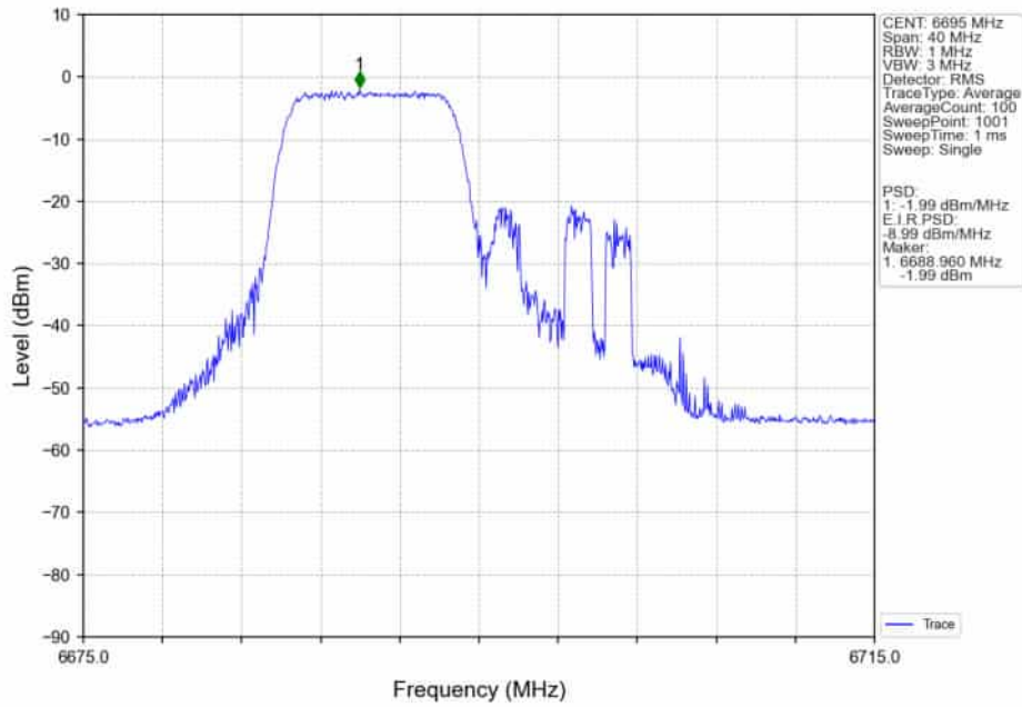
802.11ax(HEW20)_MCH_6695MHz_RU106_/_MIMO_NTNV
