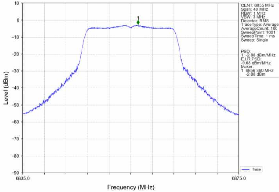
802.11a_HCH_6855MHz_Ant4_NTNV
