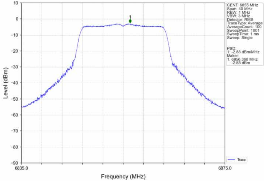
802.11a_HCH_6855MHz_Ant4_NTNV
