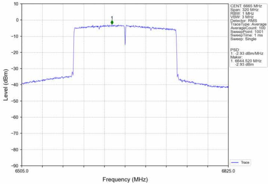
802.11ax(HEW160)_MCH_6665MHz_SU_ / _MIMO_NTNV
