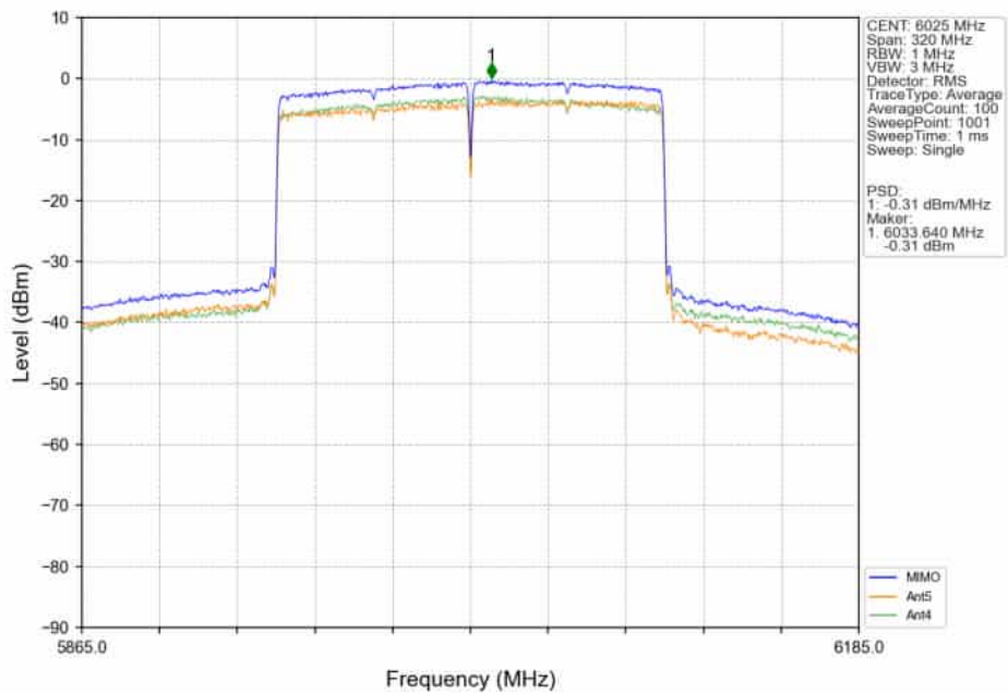
802.11ax(HEW160)_LCH_6025MHz_SU_ / _MIMO_NTNV
