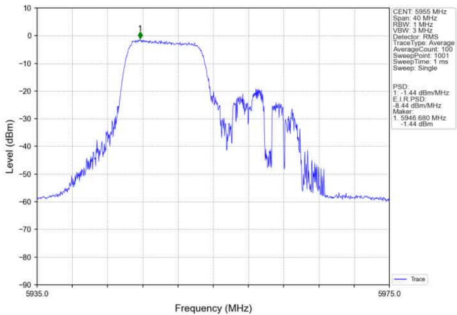
802.11ax(HEW20)_LCH_5955MHz_RU106/_Ant5_NTNV
