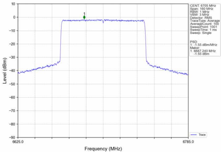
802.11ax(HEW80)_MCH_6705MHz_SU_ / _Ant5_NTNV
