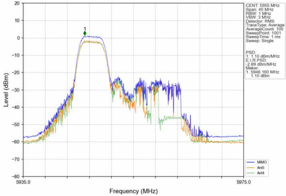
802.11ax(HEW20)_LCH_5955MHz_RU106/_Ant5_NTNV
