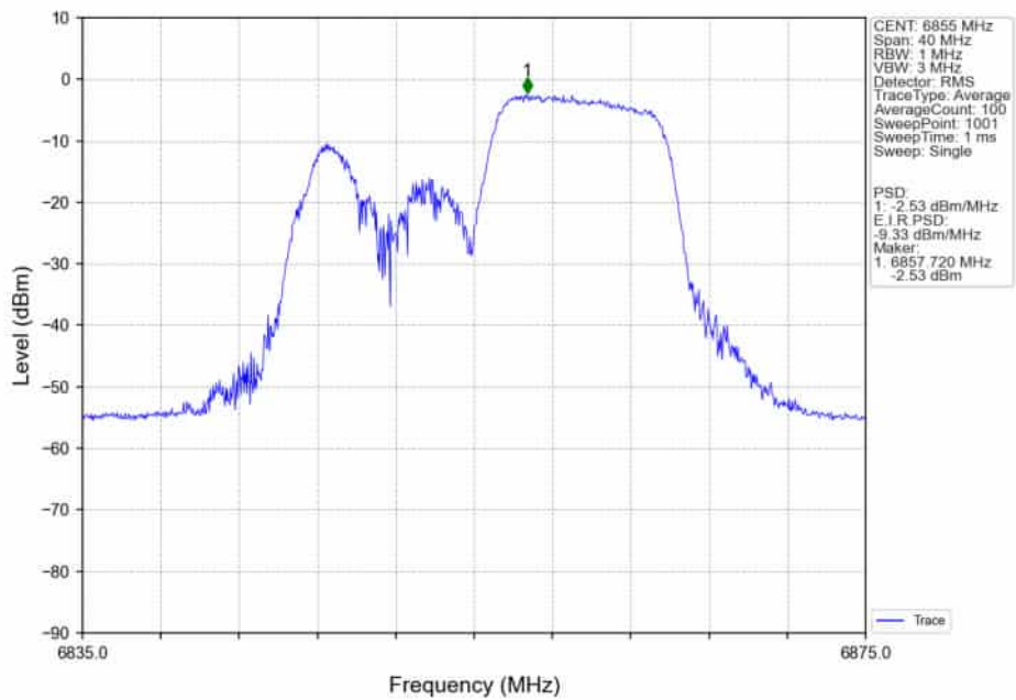
802.11ax(HEW20)_HCH_6855MHz_RU106_/_Ant5_NTNV
