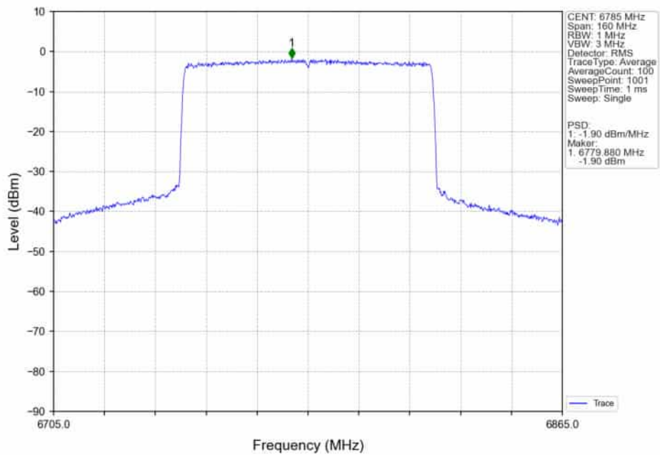
802.11ax(HEW80)_HCH_6785MHz_SU_ / _Ant4_NTNV
