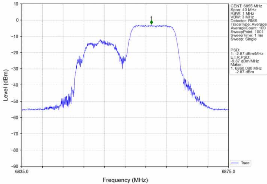
802.11ax(HEW20)_HCH_6855MHz_RU106/_MIMO_NTNV
