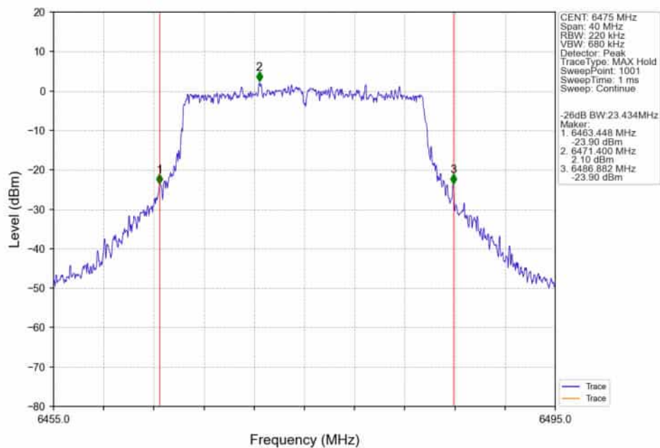
802.11ax(HEW20)_MCH_6475MHz_SU_/_Ant4_NTNV
