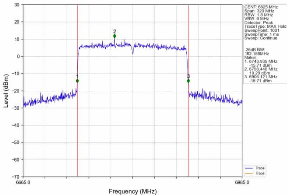
802.11ax(HEW160)_HCH_6825MHz_SU_/_Ant4_NTNV
