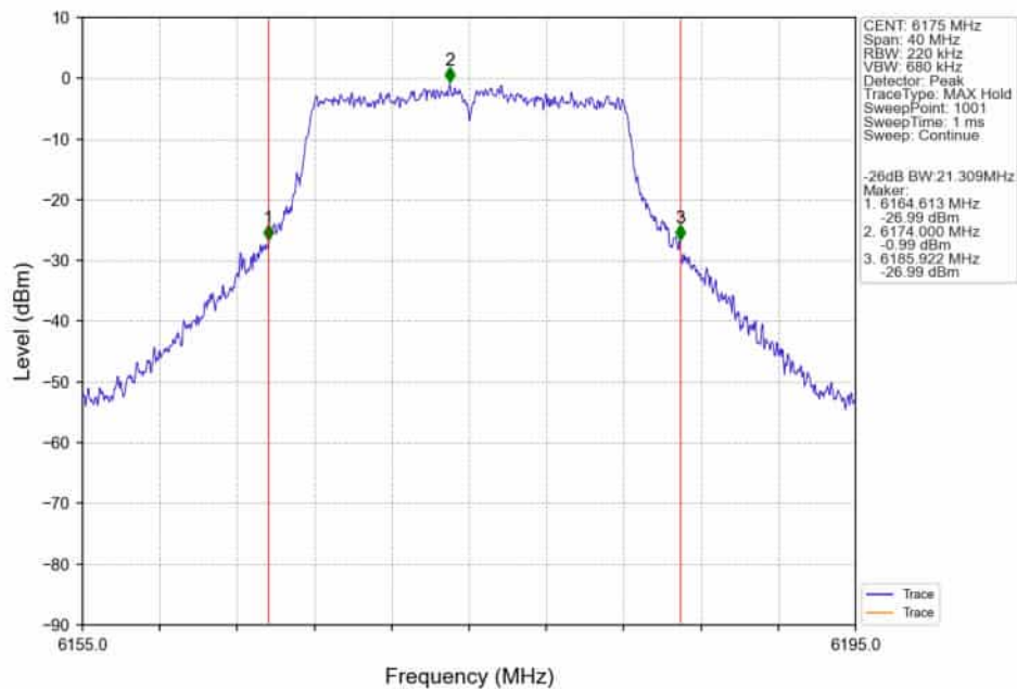
802.11a_MCH_6175MHz_Ant4_NTNV
