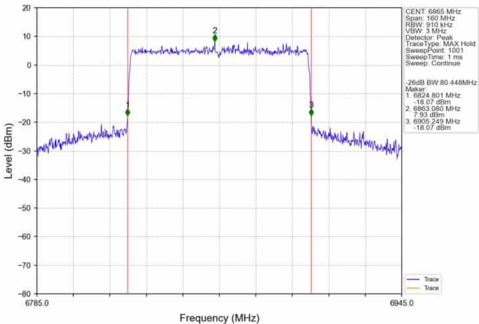
802.11ax(HEW80)_HCH_6865MHz_SU_ / Ant4_NTNV
