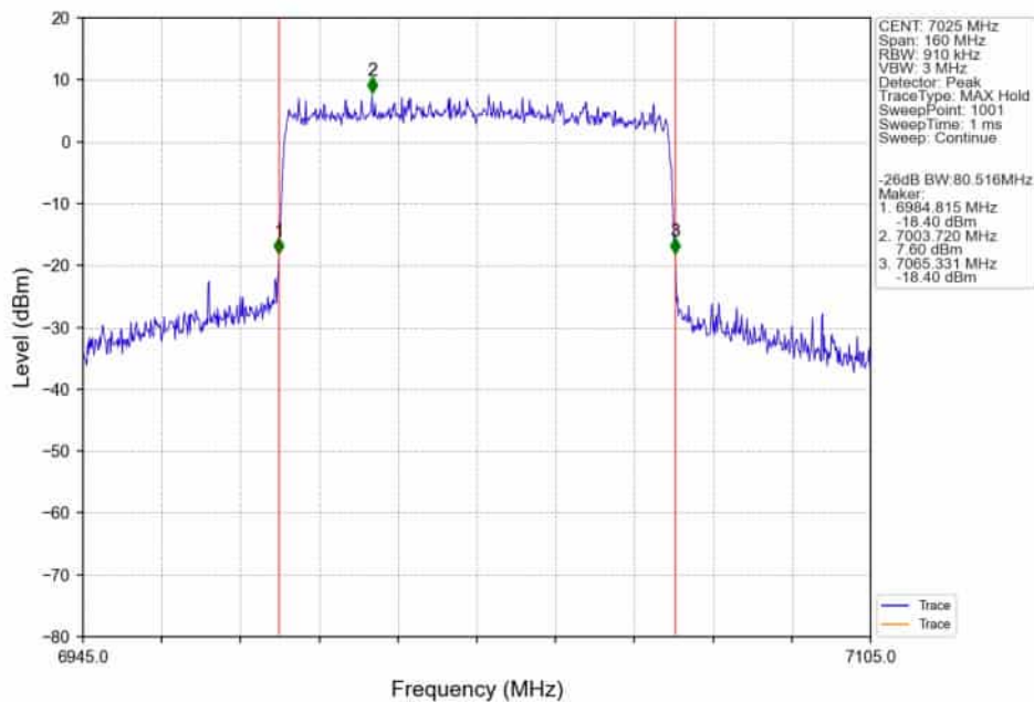
802.11ax(HEW80)_HCH_7025MHz_SU_ / Ant4_NTNV
