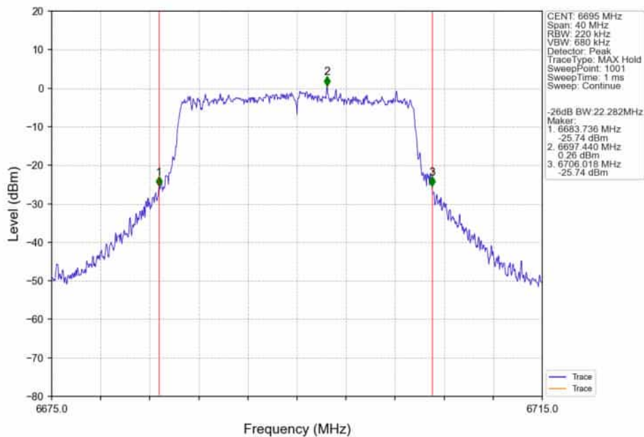
802.11ax(HEW20)_MCH_6695MHz_SU_/_Ant4_NTNV
