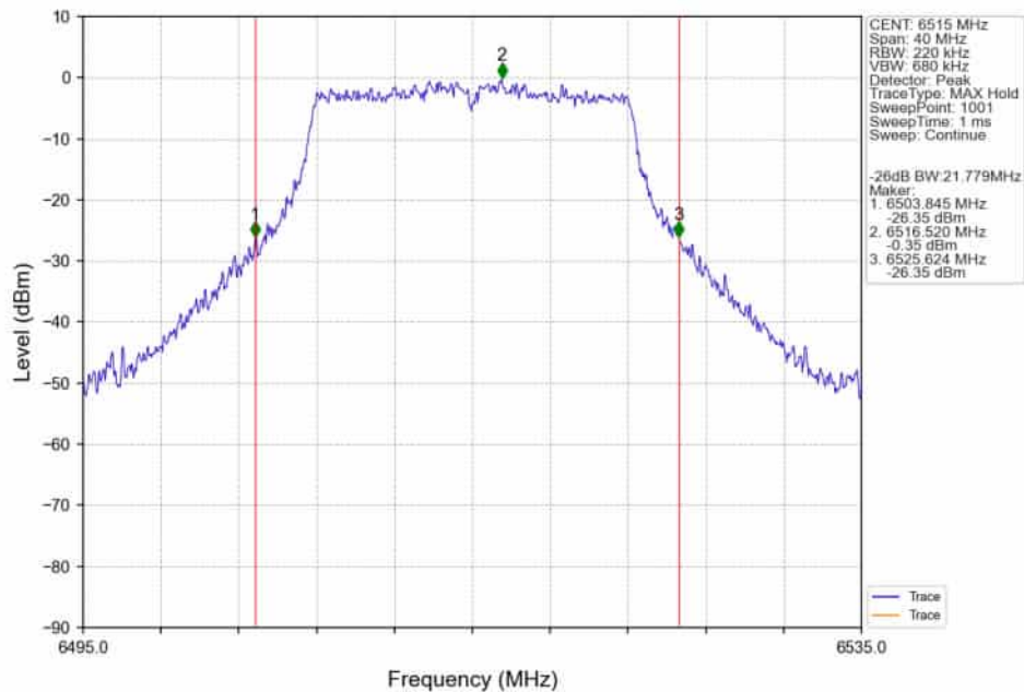
802.11a_HCH_6515MHz_Ant4_NTNV
