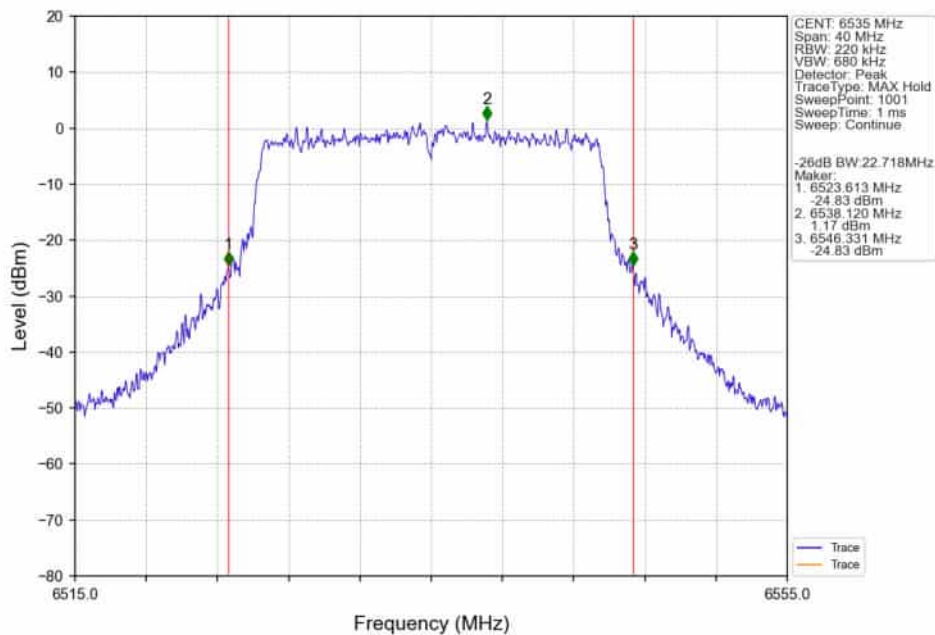
802.11ax(HEW20)_LCH_6535MHz_SU_/_Ant4_NTNV
