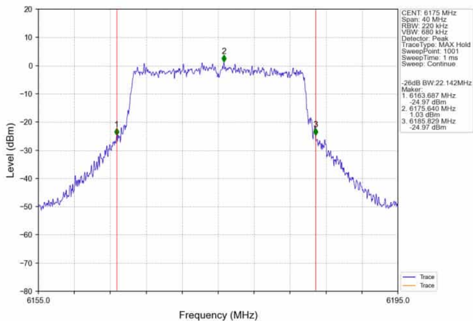
802.11ax(HEW20)_MCH_6175MHz_SU_/_Ant4_NTNV
