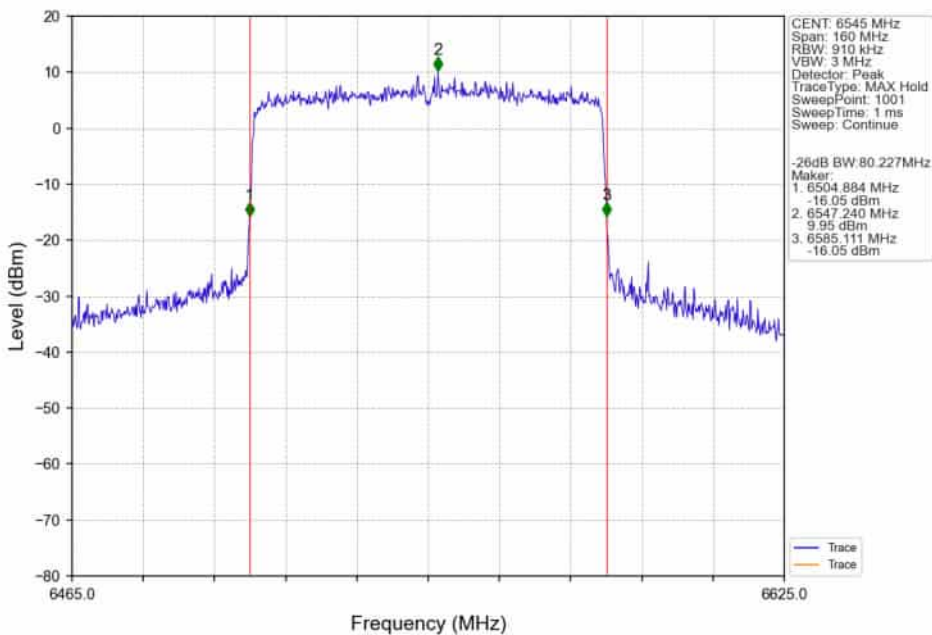
802.11ax(HEW80)_HCH_6545MHz_SU_ / Ant4_NTNV
