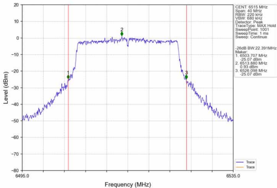
802.11ax(HEW20)_HCH_6515MHz_SU_ / Ant4_NTNV
