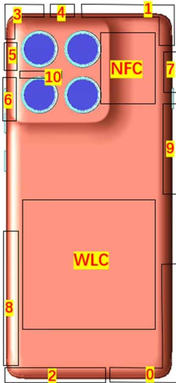
Photograph 11. Antenna position of EUT
