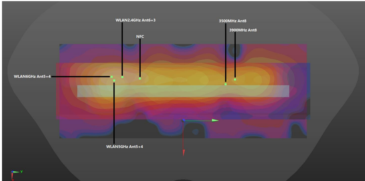
Extremity WWAN+WLAN+NFC Right Side 0mm
