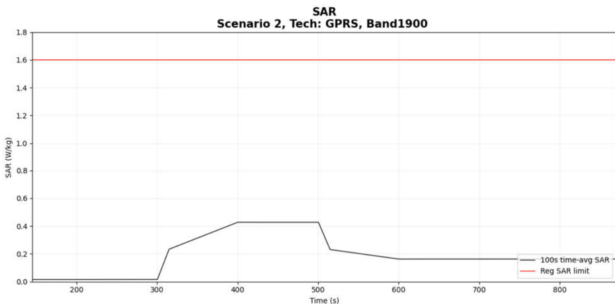
Figure 6- 5 Time-averaged SAR
