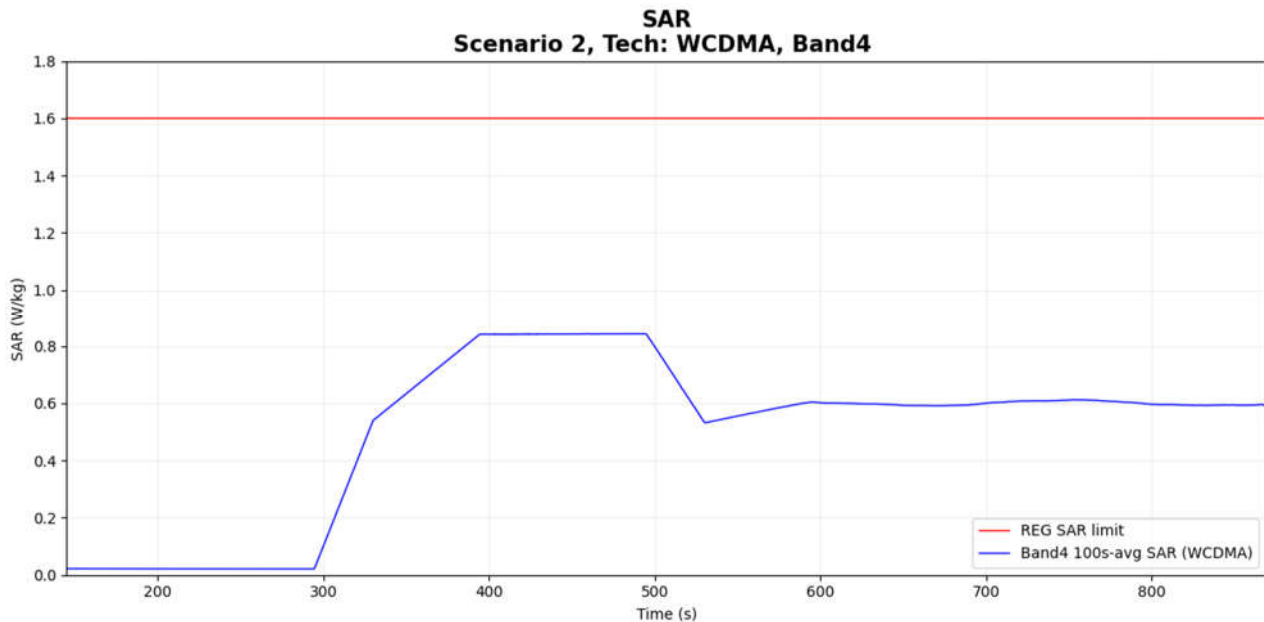
Figure 7-4 Time-averaged SAR
