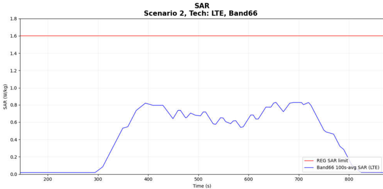
Figure 7-9 Time-averaged SAR
