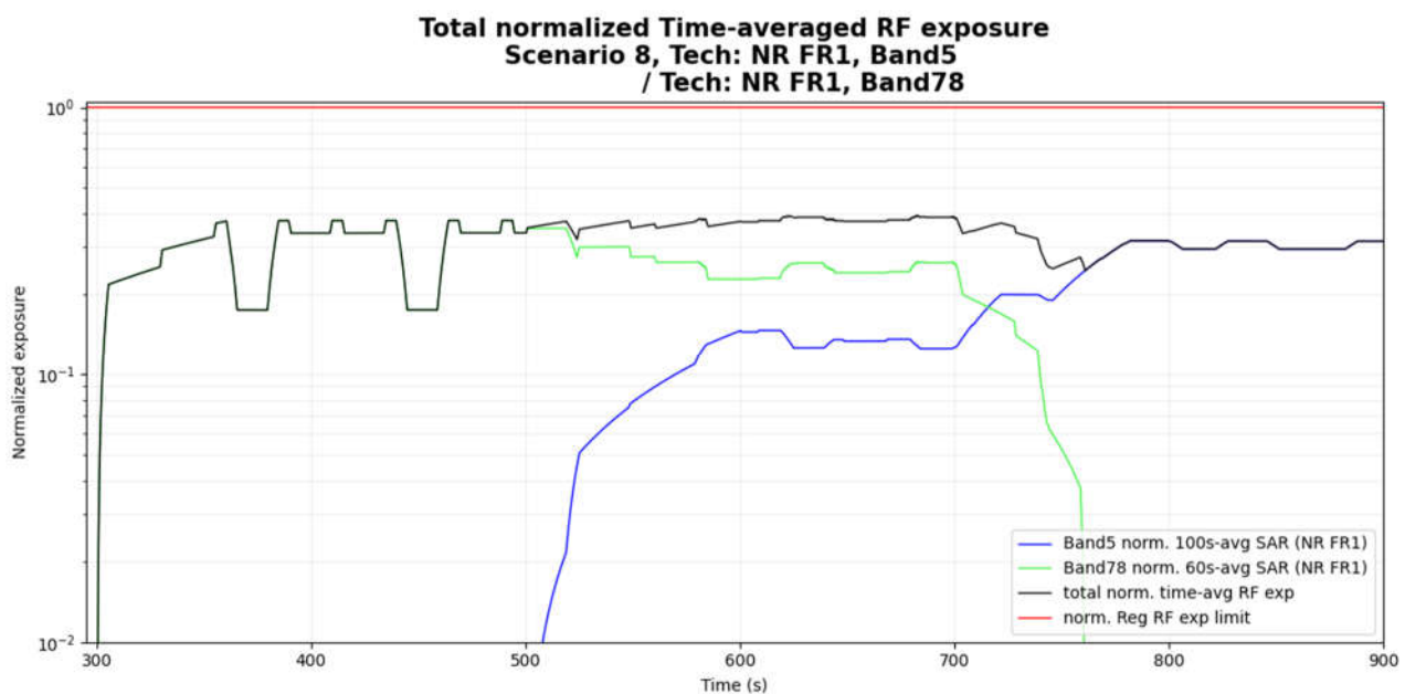
Figure 6- 25 Normalized time-averaged SAR
