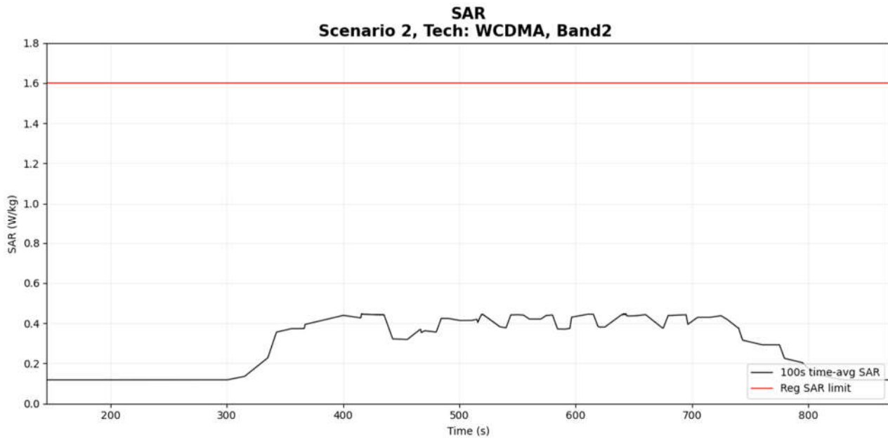
Figure 6- 10 Time-averaged SAR
