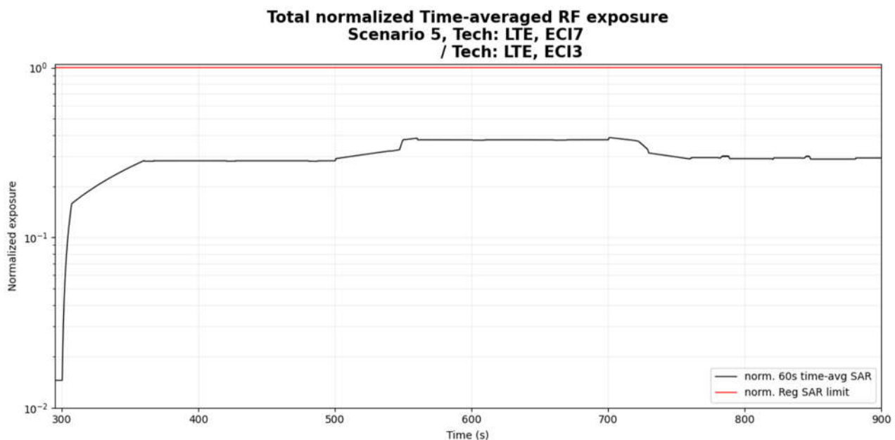
Figure 6- 21 Normalized time-averaged SAR
