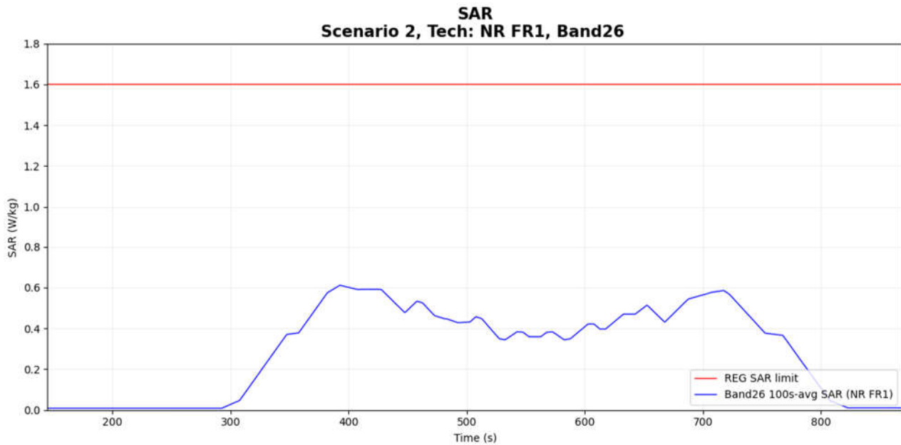
Figure 7-13 Time-averaged SAR
