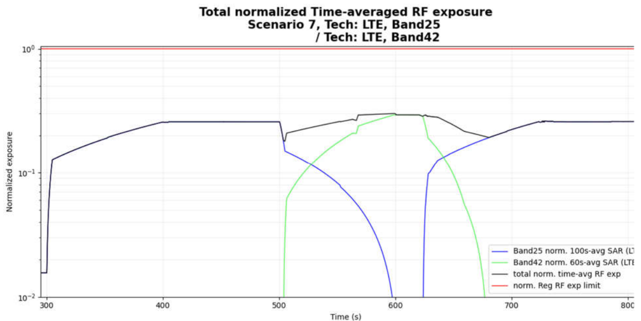
Figure 6- 23 Normalized time-averaged SAR
