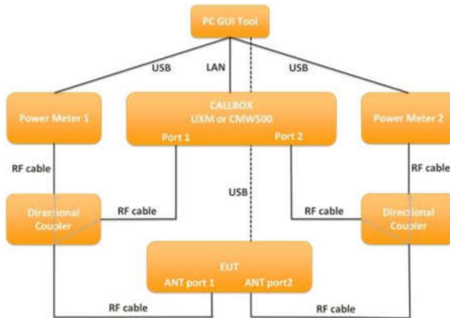
Figure 6- 3 TA-SAR conductive power test setup block diagram for scenarios 4/8
