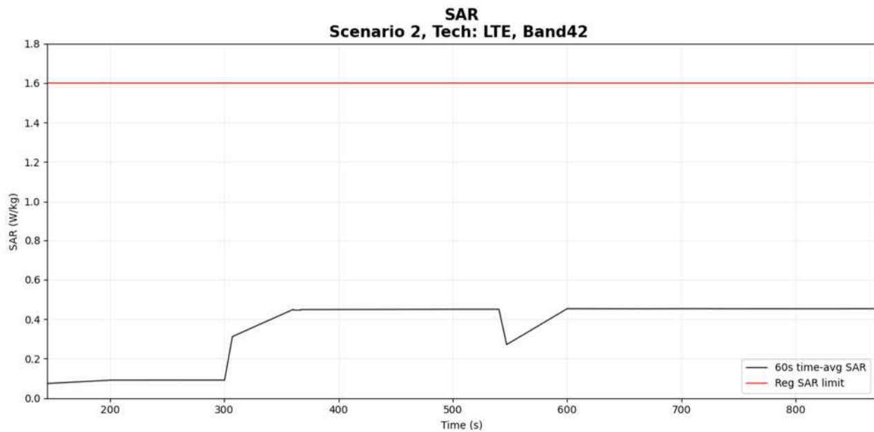
Figure 6- 13 Time-averaged SAR
