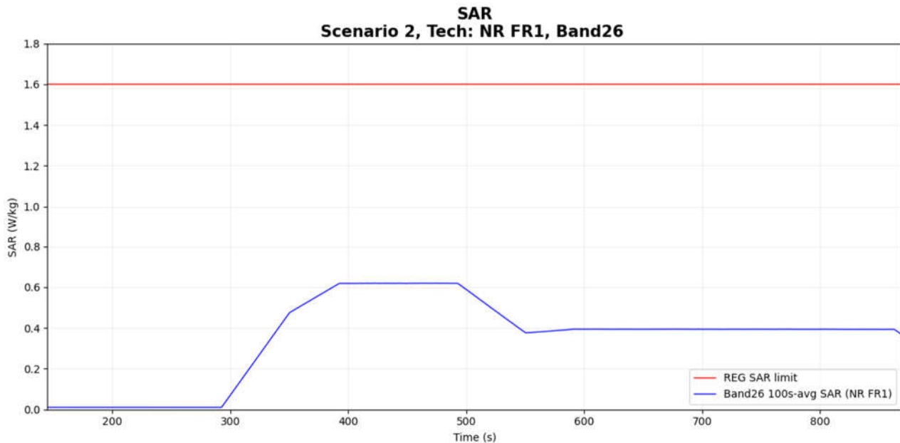
Figure 7-12 Time-averaged SAR
