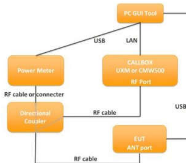
Figure 6- 1 TA-SAR conductive power test setup block diagram for scenarios 1/2/3/5
