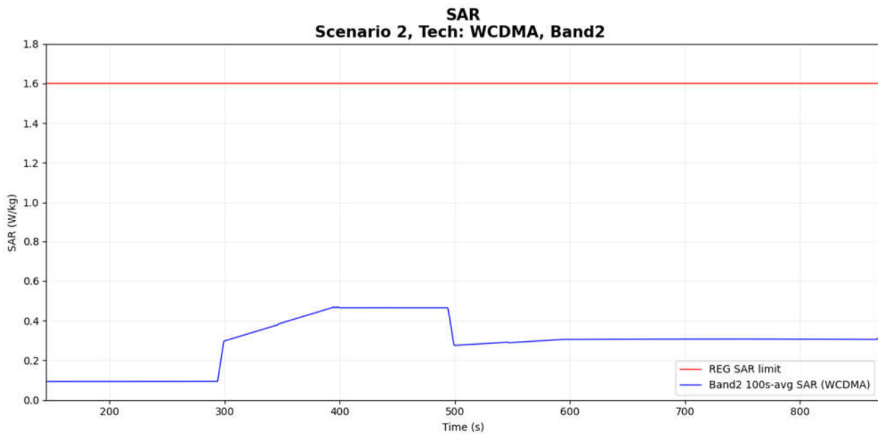
Figure 7-6 Time-averaged SAR
