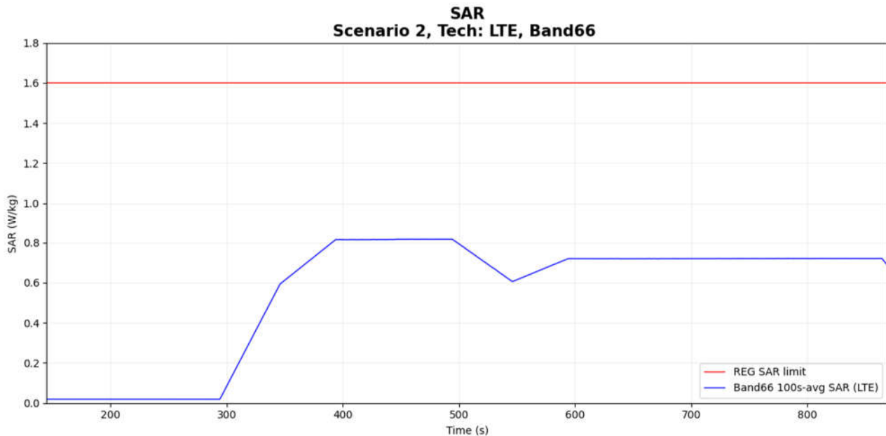
Figure 7-8 Time-averaged SAR
