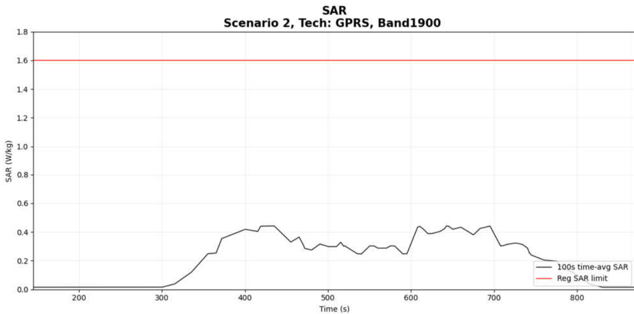
Figure 6- 6 Time-averaged SAR
