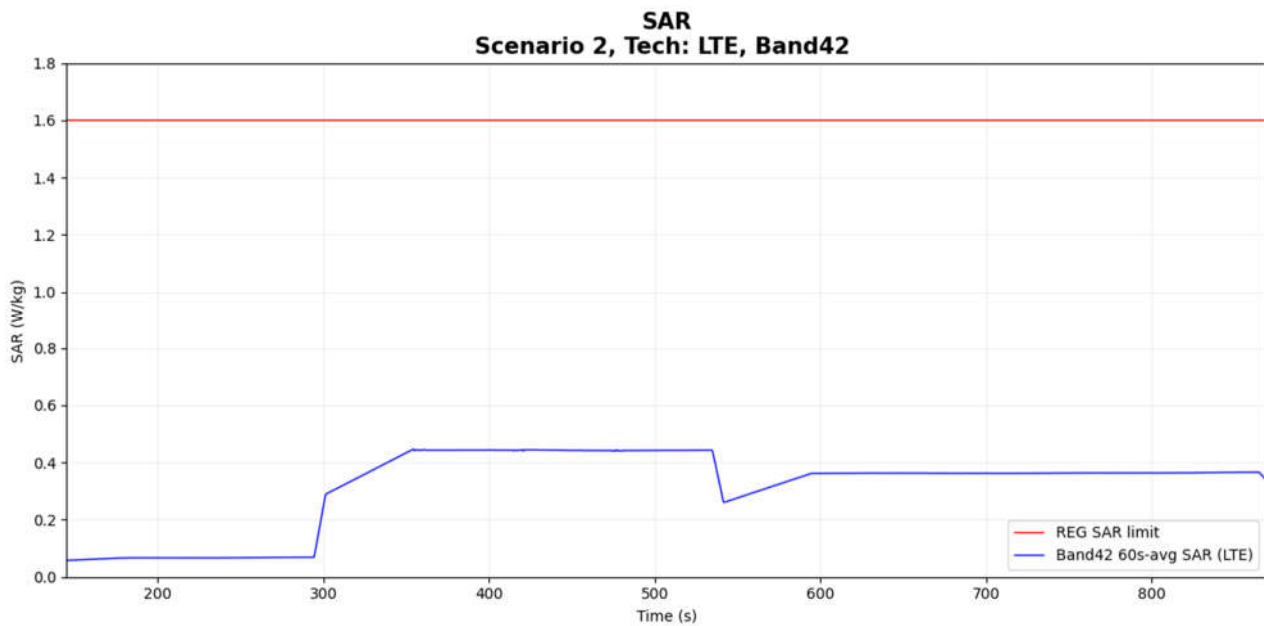
Figure 7-10 Time-averaged SAR
