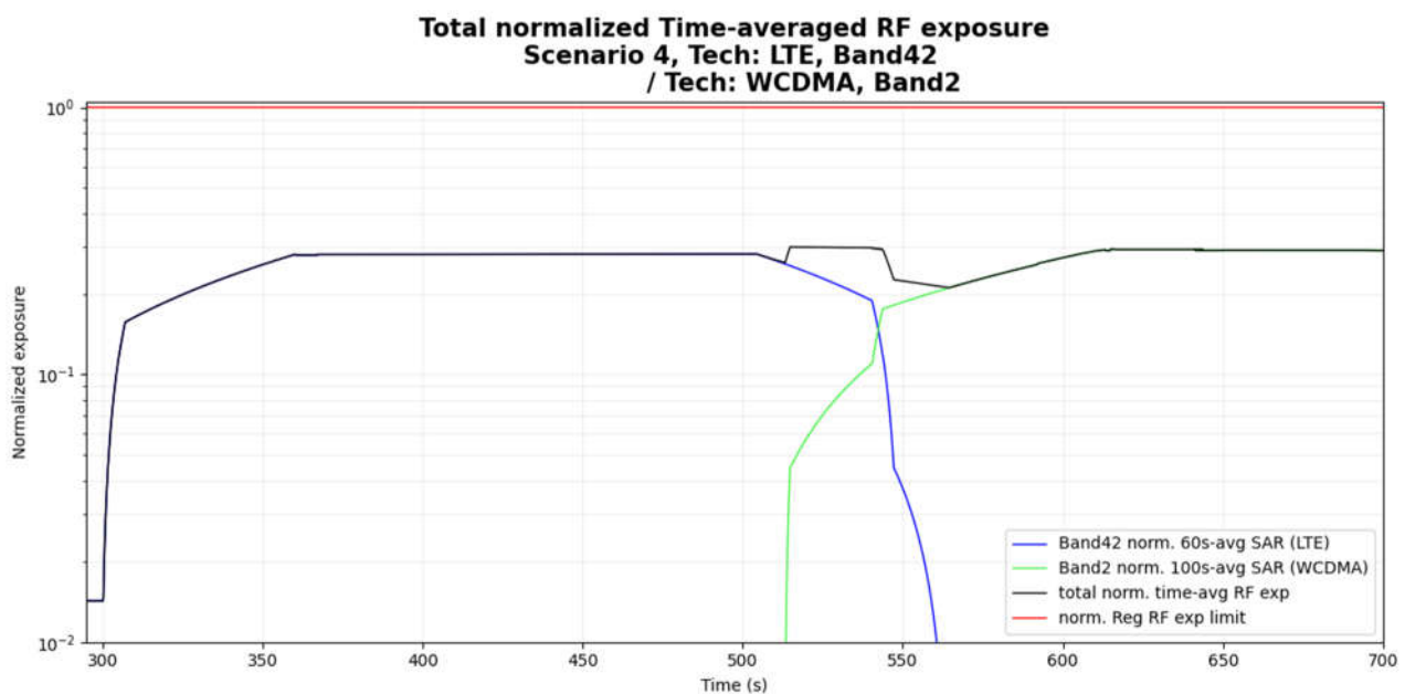
Figure 6- 20 Normalized time-averaged SAR
