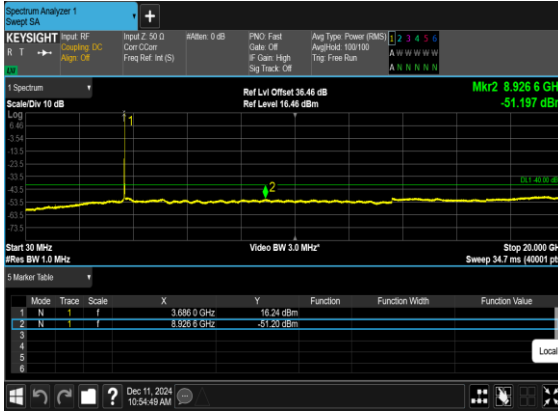
N48(15M)_CP-OFDM_QPSK_Edge_1RB_Left_High_CH
