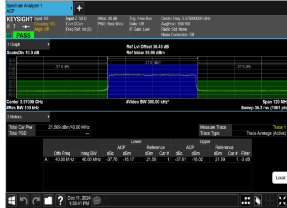
N48(40M)_CP-OFDM_16QAM_Outer_Full_Low_CH
