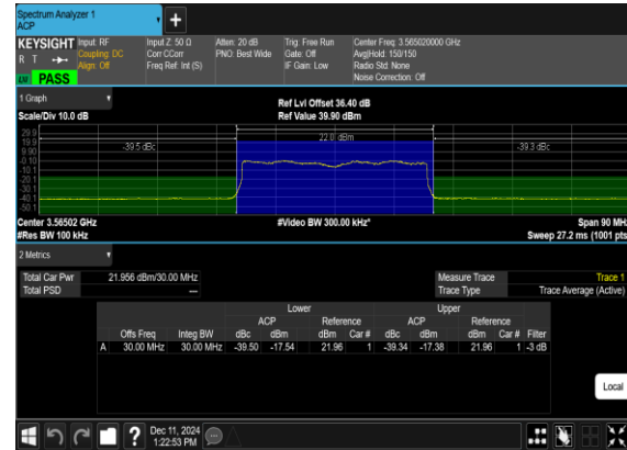
N48(30M)_CP-OFDM_16QAM_Outer_Full_Low_CH
