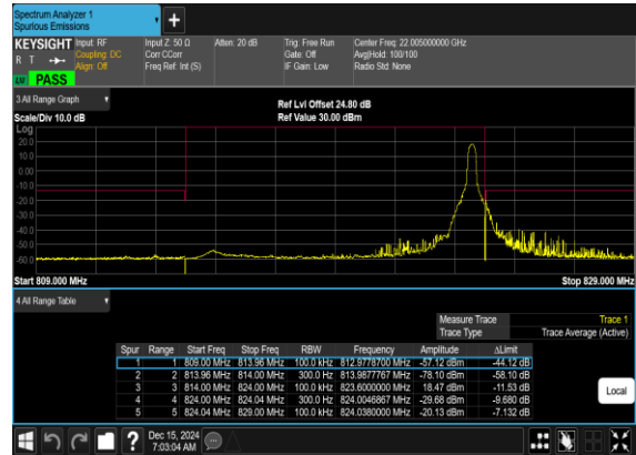
N26(10M)_DFT-s-OFDM_QPSK_Edge_1RB_Right_Mid_CH
