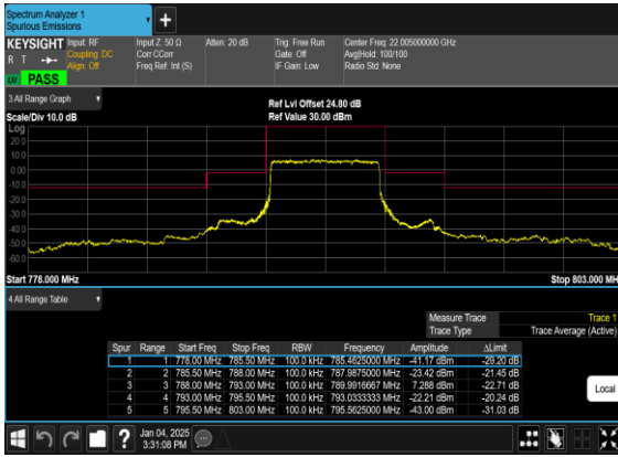
N14(5M)_DFT-s-OFDM_BPSK_Outer_Full_Low_CH
