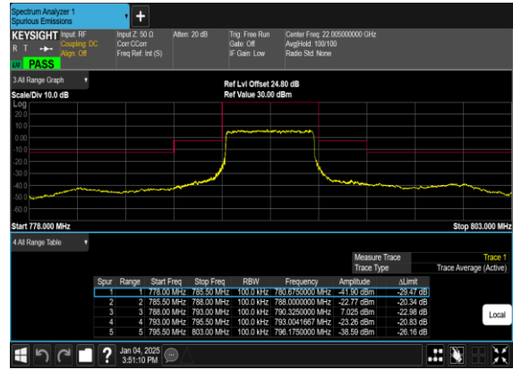
N14(5M)_DFT-s-OFDM_QPSK_Outer_Full_Low_CH
