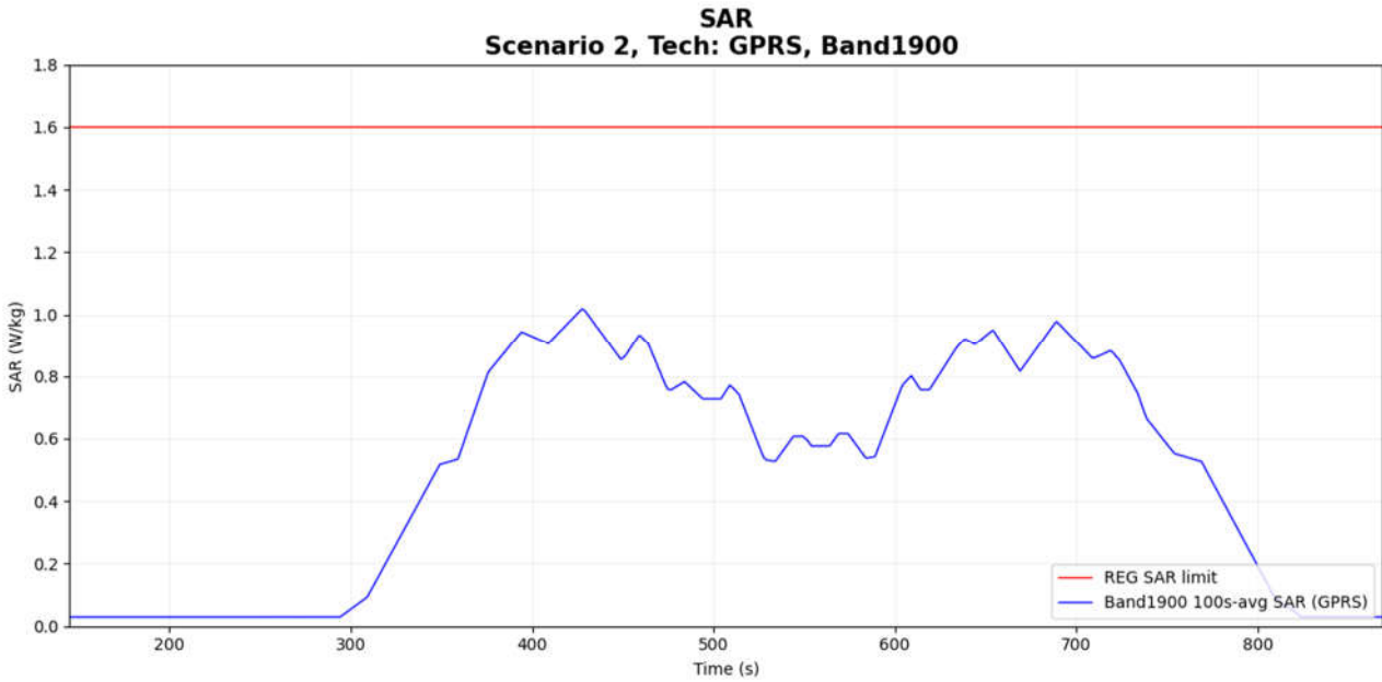
Figure 7-5 Time-averaged SAR
