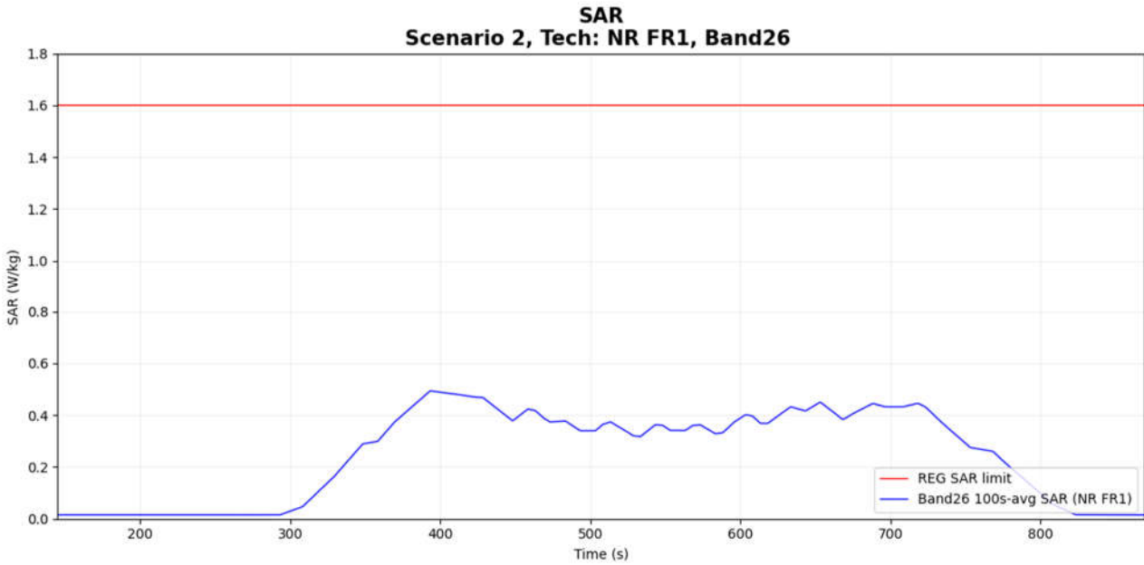
Figure 7-15 Time-averaged SAR
