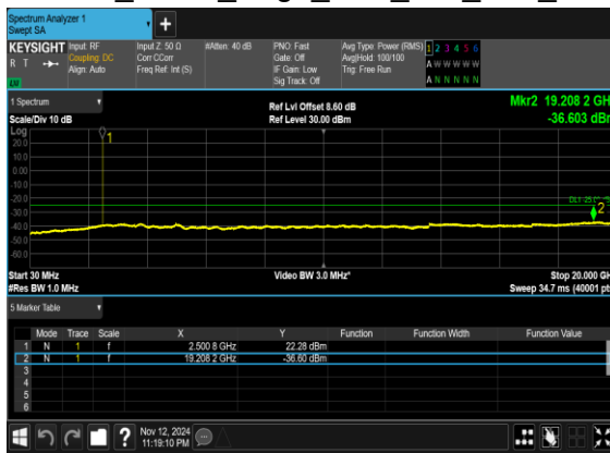
N7(20M)_DFT-s- OFDM_BPSK_Edge_1RB_Left_Low_CH
