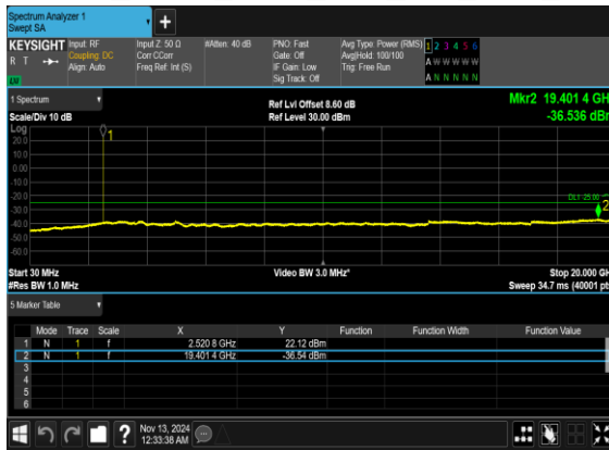
N7(50M)_DFT-s- OFDM_BPSK_Edge_1RB_Left_High_CH
