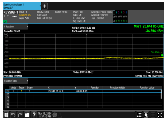
N7(50M)_DFT-s- OFDM_QPSK_Edge_1RB_Left_High_CH
