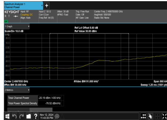
N7(20M)_DFT-s- OFDM_BPSK_Edge_1RB_Left_Low_CH_CHP_PASS
