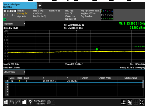
N7(20M)_DFT-s- OFDM_BPSK_Edge_1RB_Left_Low_CH
