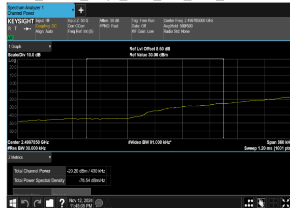
N7(20M)_DFT-s- OFDM_QPSK_Edge_1RB_Left_Low_CH_CHP_PASS
