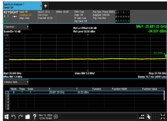
N7(50M)_DFT-s- OFDM_BPSK_Edge_1RB_Left_High_CH
