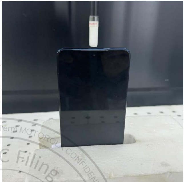
Top Side, Test Separation 2 mm
