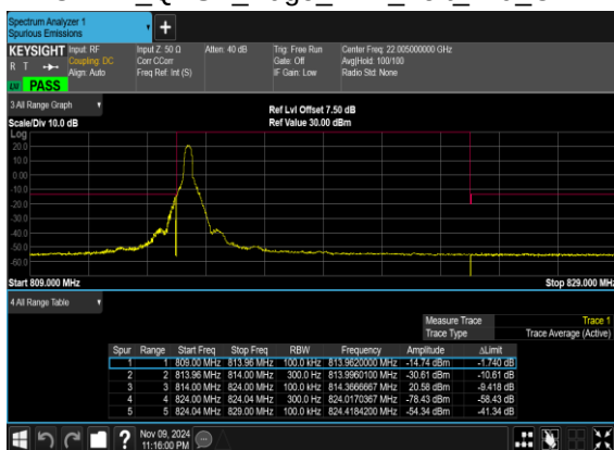
N26(10M)_DFT-s- OFDM_QPSK_Edge_1RB_Left_Mid_CH
