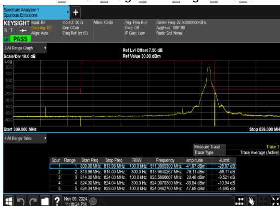
N26(10M)_DFT-s- OFDM_BPSK_Edge_1RB_Right_Mid_CH
