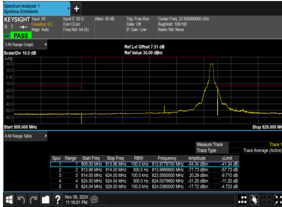
N26(10M)_DFT-s- OFDM_QPSK_Edge_1RB_Right_Mid_CH
