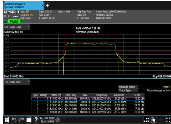
N26(5M)_DFT-s- OFDM_BPSK_Outer_Full_High_CH
