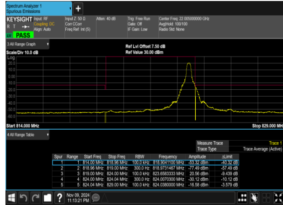
N26(5M)_DFT-s- OFDM_BPSK_Edge_1RB_Right_High_CH
