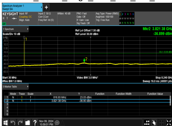
N26(5M)_DFT-s-OFDM_BPSK_Edge_1RB_Left_Mid_CH
