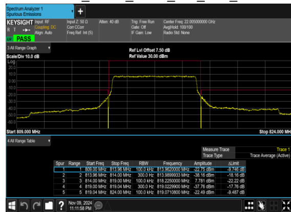
N26(5M)_DFT-s-OFDM_BPSK_Outer_Full_Low_CH
