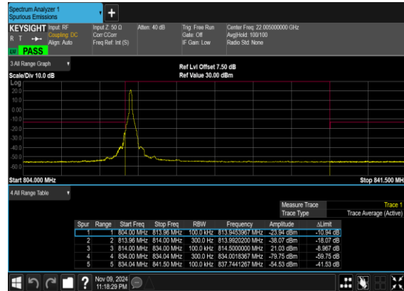
N26(20M)_DFT-s- OFDM_BPSK_Edge_1RB_Left_Mid_CH
