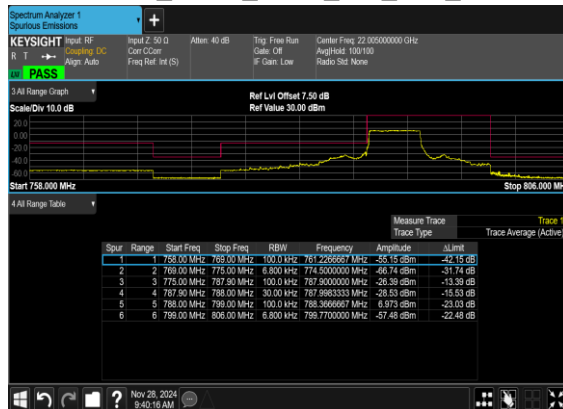
N14(5M)_DFT-s- OFDM_BPSK_Outer_Full_Low_CH
