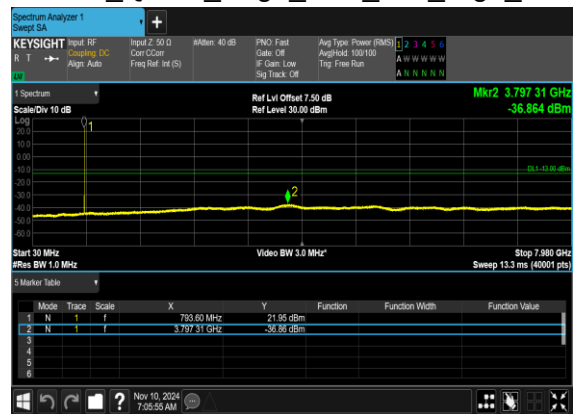
N14(5M)_DFT-s- OFDM_QPSK_Edge_1RB_Left_High_CH
