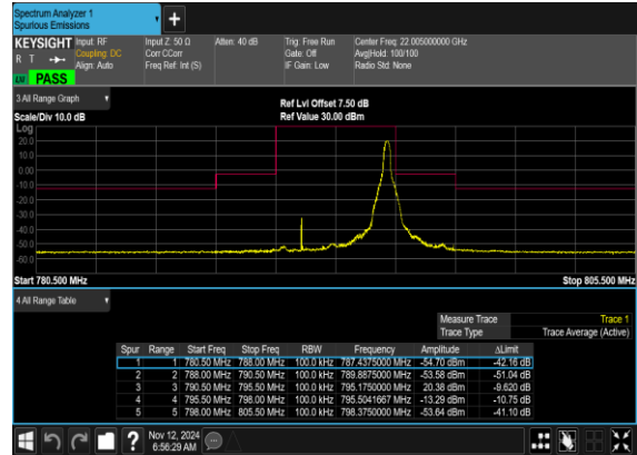
N14(5M)_DFT-s- OFDM_QPSK_Edge_1RB_Right_Mid_CH
