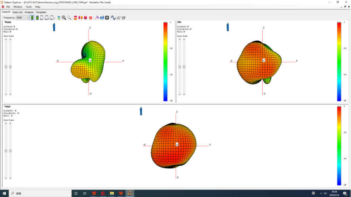
Wifi CHAIN1 5g w56
