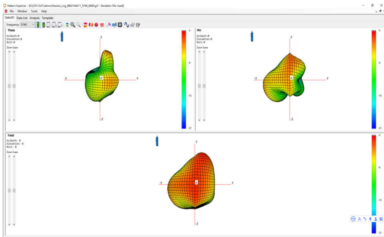
Wifi CHAIN1 5g 5.8G
