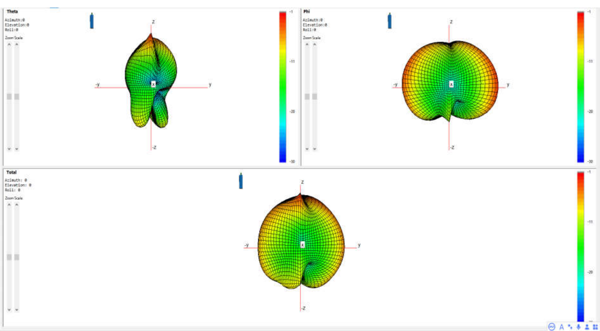
Wifi CHAIN0 5g w53
