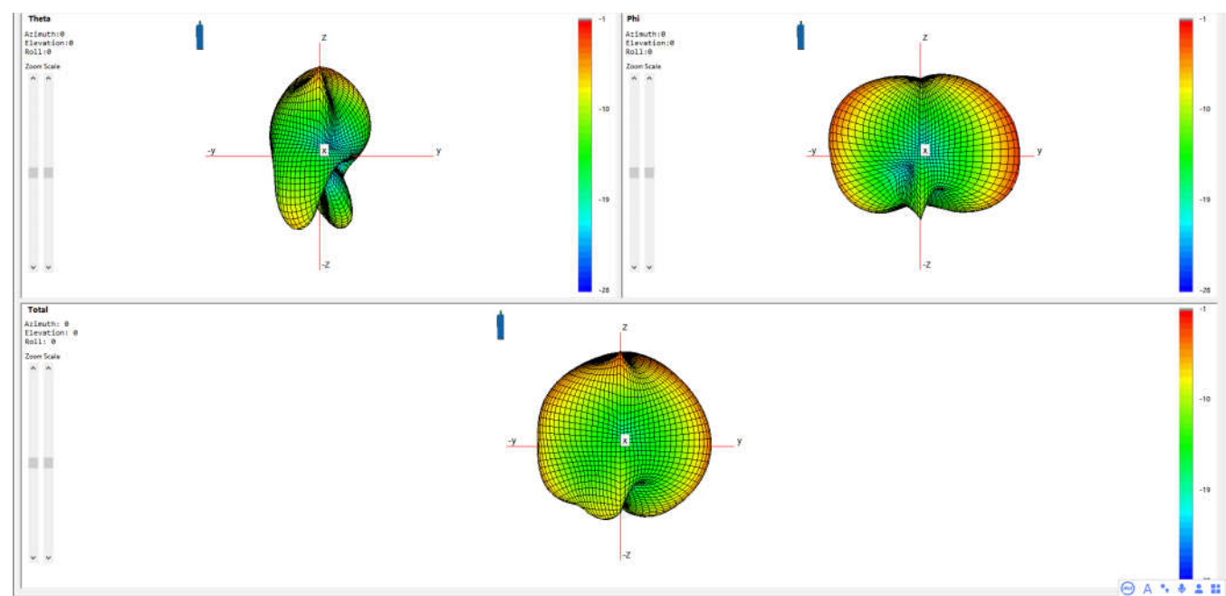
Wifi CHAIN0 5g w52
