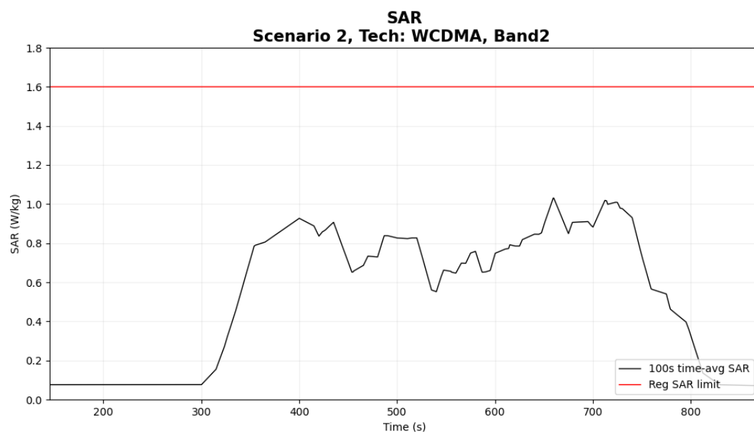
Figure 5- 17 Time-averaged SAR
