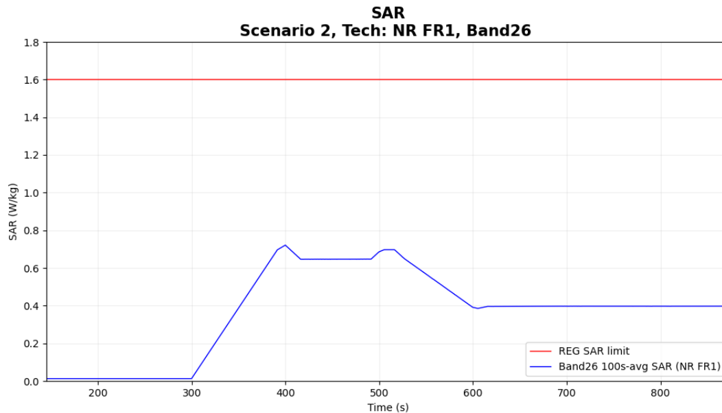
Figure 6-3 Time-averaged SAR
