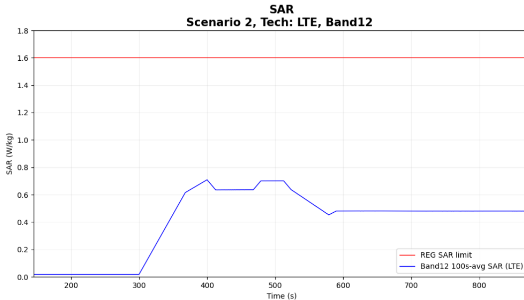
Figure 6-7 Time-averaged SAR
