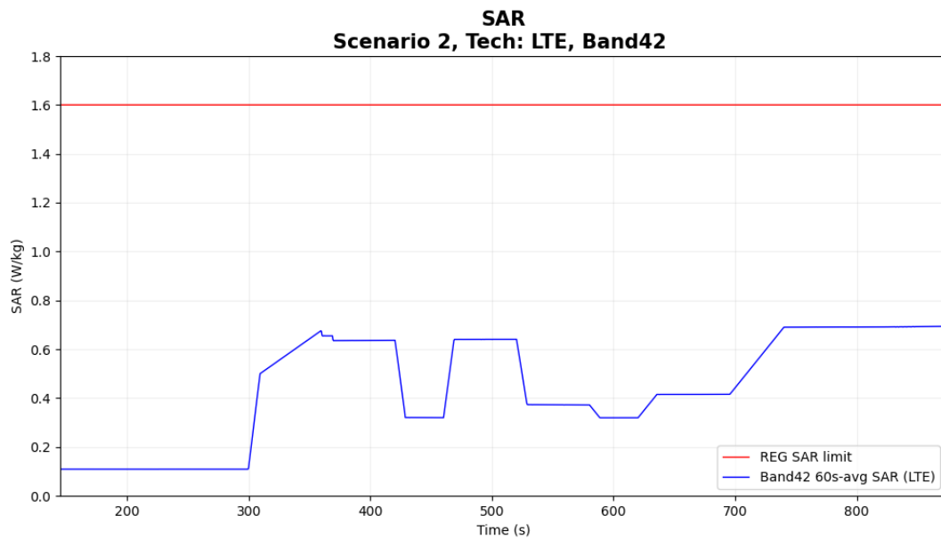
Figure 6-9 Time-averaged SAR
