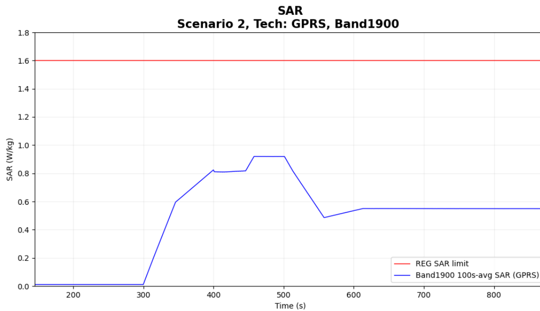
Figure 6-17 Time-averaged SAR
