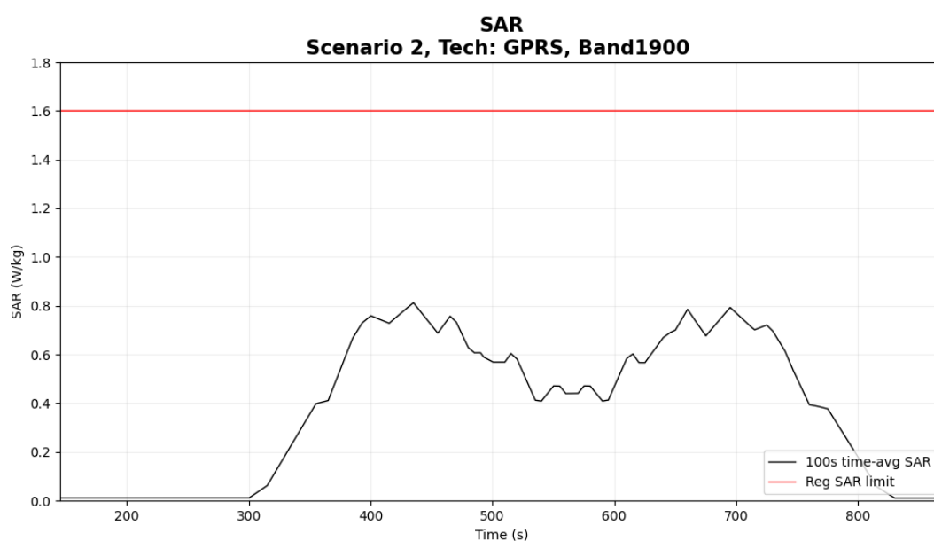
Figure 5- 14 Time-averaged SAR
