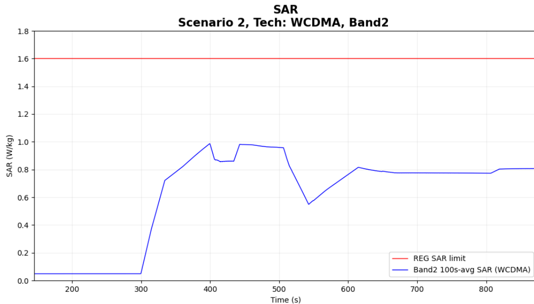
Figure 6-11 Time-averaged SAR
