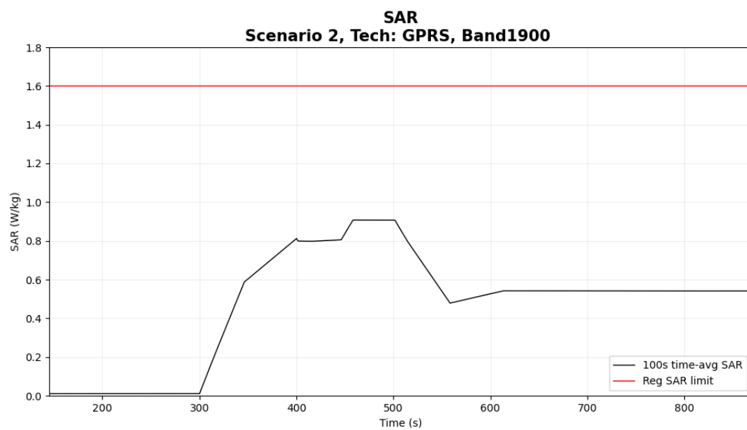
Figure 5- 12 Time-averaged SAR
