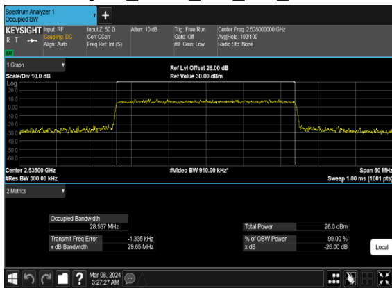
N7(30M)_CP-OFDM_16 QAM_Outer_Full_Mid_CH
