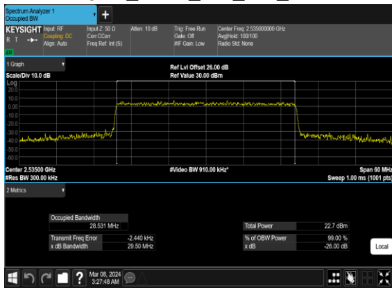
N7(30M)_CP-OFDM_256 QAM_Outer_Full_Mid_CH
