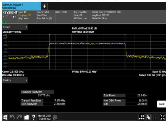
N7(25M)_CP-OFDM_256 QAM_Outer_Full_Mid_CH
