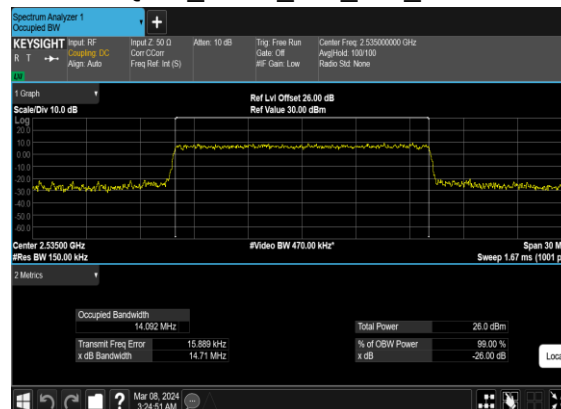
N7(15M)_CP-OFDM_16 QAM_Outer_Full_Mid_CH
