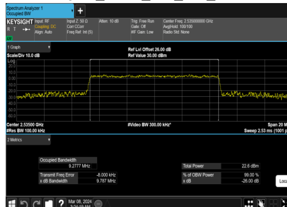
N7(10M)_CP-OFDM_256 QAM_Outer_Full_Mid_CH
