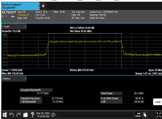
N70(15M)_CP-OFDM_64 QAM_Outer_Full_Mid_CH
