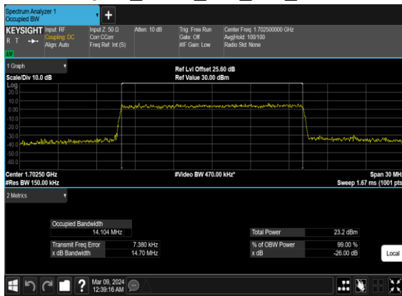
N70(15M)_CP-OFDM_256 QAM_Outer_Full_Mid_CH
