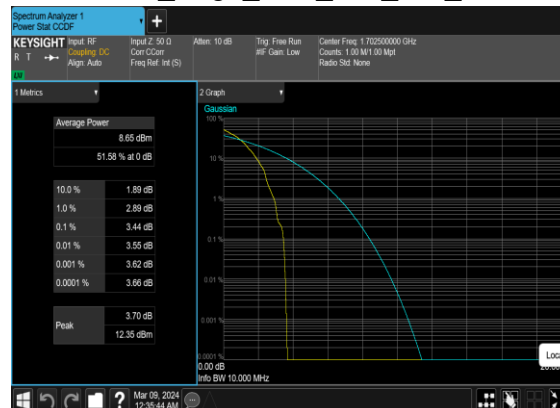
N70(15M)_DFT-s-OFDM_PI_2- BPSK_Edge_1RB_Left_Mid_CH
