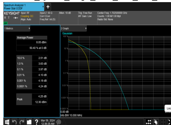
N70(15M)_DFT-s- OFDM_QPSK_Edge_1RB_Left_Mid_CH
