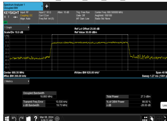
N71(20M)_CP-OFDM_16 QAM_Outer_Full_Mid_CH
