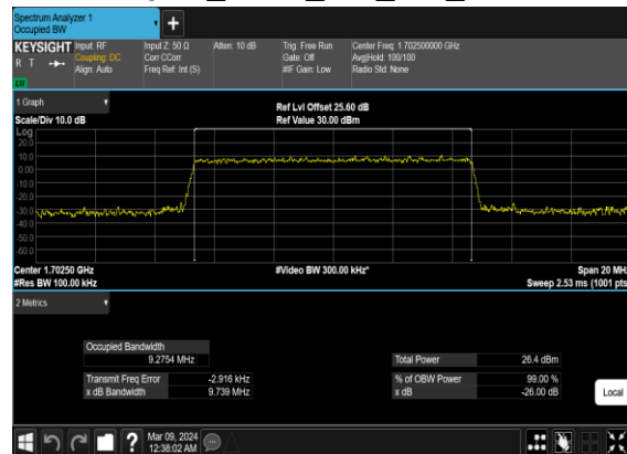
N70(10M)_CP-OFDM_16 QAM_Outer_Full_Mid_CH
