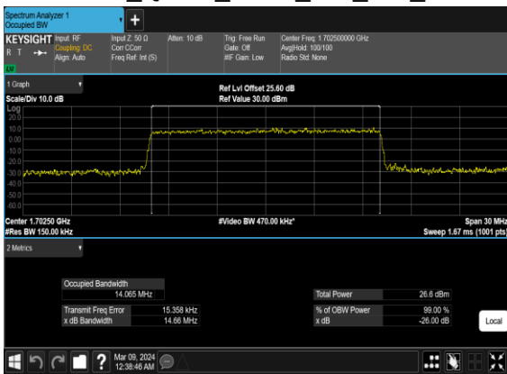
N70(15M)_CP- OFDM_QPSK_Outer_Full_Mid_CH
