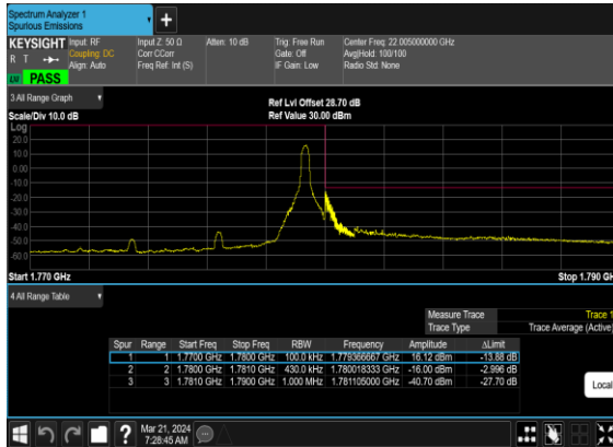
N66(40M)_CP- OFDM_QPSK_Edge_1RB_Right_High_CH
