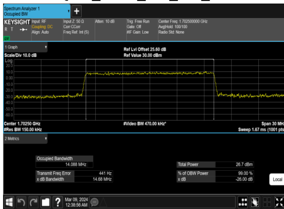
N70(15M)_CP-OFDM_16 QAM_Outer_Full_Mid_CH
