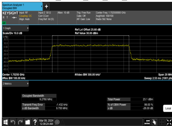
N70(10M)_CP-OFDM_256 QAM_Outer_Full_Mid_CH
