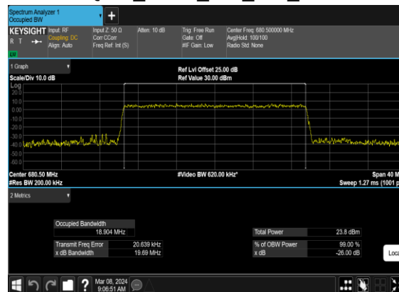
N71(20M)_CP-OFDM_256 QAM_Outer_Full_Mid_CH
