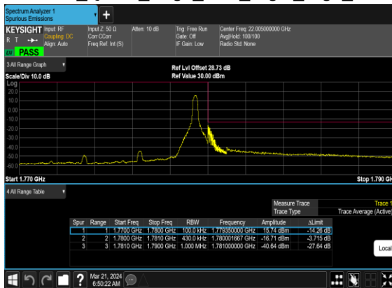
N66(40M)_CP- OFDM_QPSK_Edge_1RB_Right_High_CH
