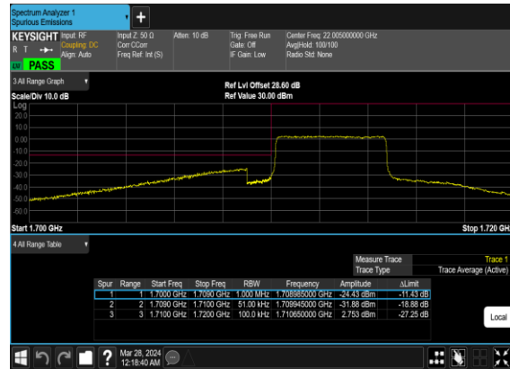
N66(5M)_CP-OFDM_16 QAM_Outer_Full_Low_CH
