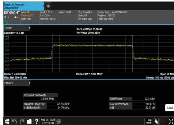
N66(35M)_CP-OFDM_256 QAM_Outer_Full_Mid_CH
