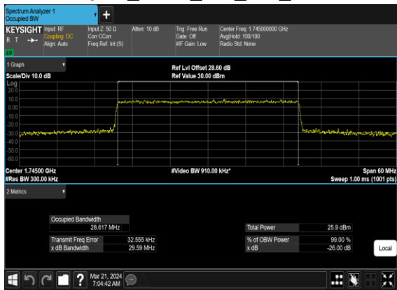
N66(30M)_CP-OFDM_64 QAM_Outer_Full_Mid_CH
