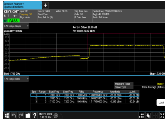
N66(10M)_CP-OFDM_16 QAM_Outer_Full_Low_CH
