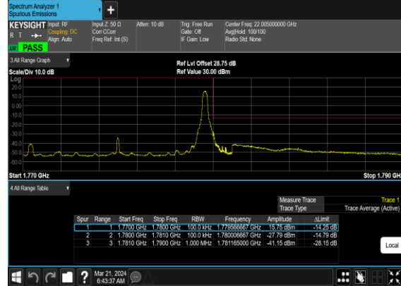
N66(10M)_CP-OFDM_16 QAM_Edge_1RB_Right_High_CH
