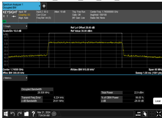
N66(30M)_CP-OFDM_256 QAM_Outer_Full_Mid_CH
