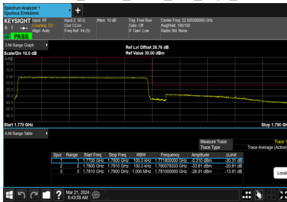
N66(10M)_CP- OFDM_QPSK_Outer_Full_High_CH
