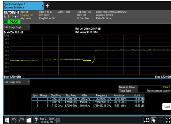
N66(40M)_CP-OFDM_16 QAM_Outer_Full_Low_CH
