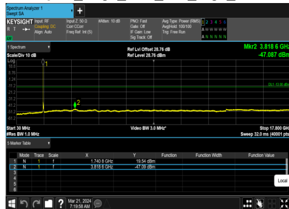
N66(40M)_CP-OFDM_16 QAM_Edge_1RB_Left_High_CH
