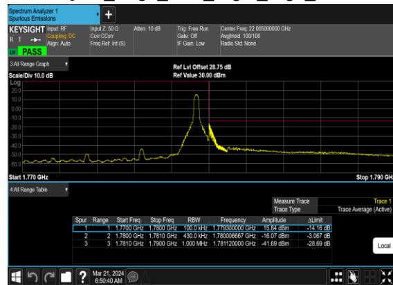
N66(40M)_CP-OFDM_16 QAM_Edge_1RB_Right_High_CH
