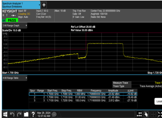
N66(5M)_CP- OFDM_QPSK_Outer_Full_Low_CH
