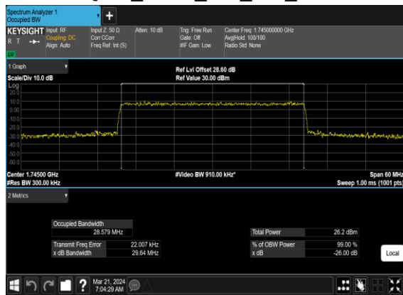
N66(30M)_CP-OFDM_16 QAM_Outer_Full_Mid_CH
