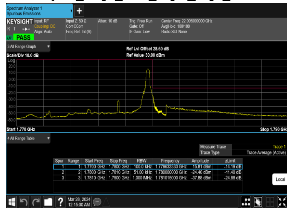
N66(5M)_CP-OFDM_16 QAM_Edge_1RB_Right_High_CH
