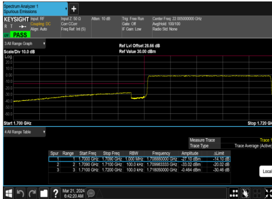
N66(10M)_CP- OFDM_QPSK_Outer_Full_Low_CH
