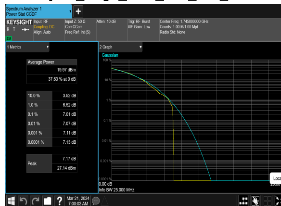
N66(20M)_CP-OFDM_16 QAM_Edge_1RB_Left_Mid_CH
