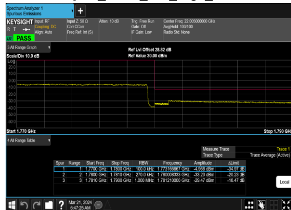
N66(25M)_CP-OFDM_16 QAM_Outer_Full_High_CH
