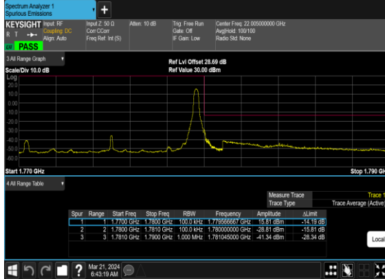
N66(10M)_CP- OFDM_QPSK_Edge_1RB_Right_High_CH
