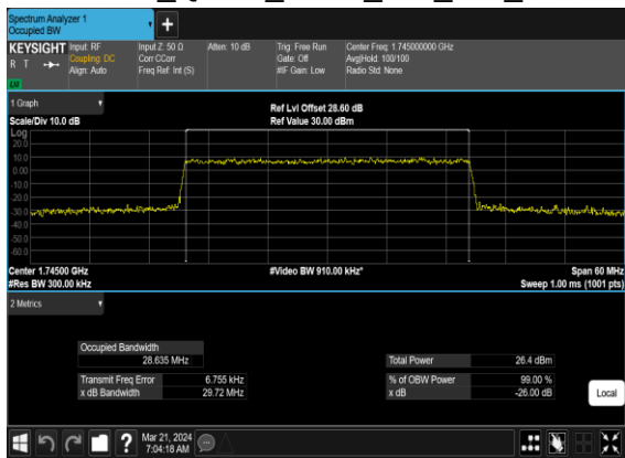
N66(30M)_CP- OFDM_QPSK_Outer_Full_Mid_CH
