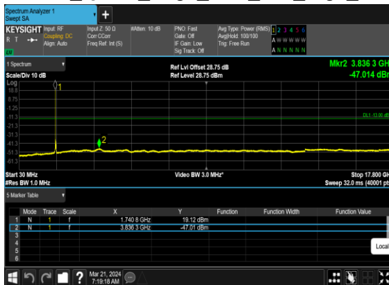
N66(40M)_CP- OFDM_QPSK_Edge_1RB_Left_High_CH
