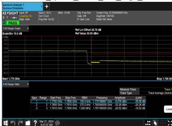
N66(25M)_CP- OFDM_QPSK_Outer_Full_High_CH
