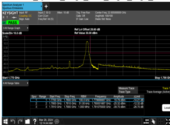
N66(5M)_CP- OFDM_QPSK_Edge_1RB_Right_High_CH
