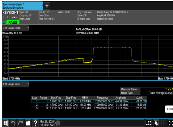
N66(5M)_CP- OFDM_QPSK_Outer_Full_Low_CH
