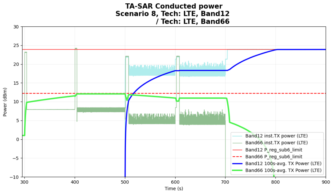
Figure 5- 48 Time-averaged conducted TX power over time
