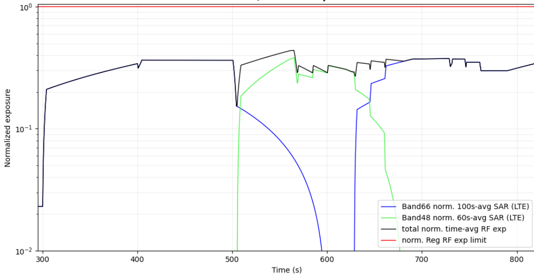
Figure 5- 45 Normalized time-averaged SAR
