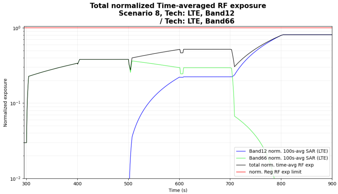
Figure 5- 49 Normalized time-averaged SAR
