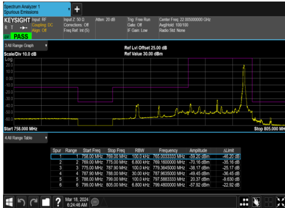
N14(10M)_DFT-s- OFDM_BPSK_Edge_1RB_Right_Mid_CH
