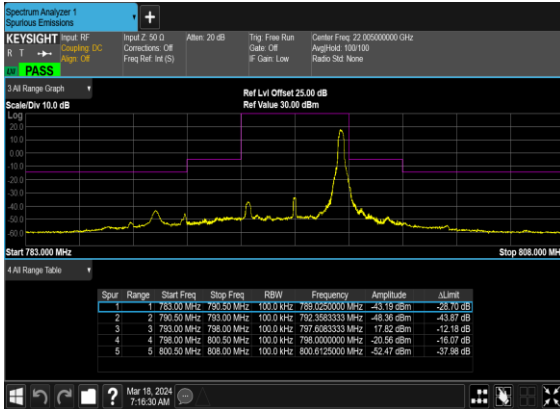
N14(5M)_CP- OFDM_QPSK_Edge_1RB_Right_High_CH
