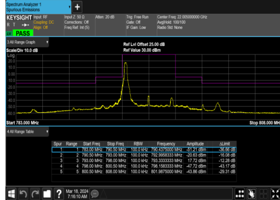
N14(5M)_CP-OFDM_16 QAM_Edge_1RB_Left_High_CH
