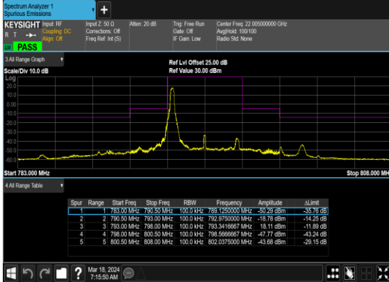
N14(5M)_CP- OFDM_QPSK_Edge_1RB_Left_High_CH
