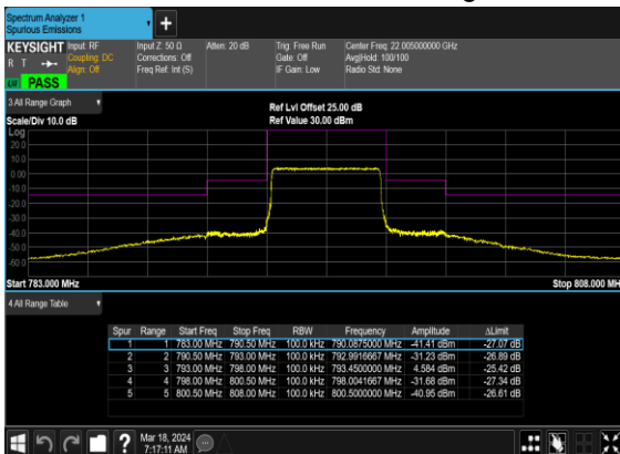
N14(5M)_CP- OFDM_QPSK_Outer_Full_High_CH
