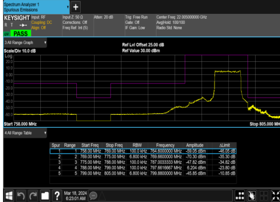
N14(5M)_DFT-s- OFDM_BPSK_Outer_Full_High_CH
