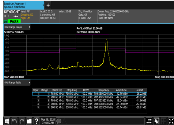
N14(5M)_CP-OFDM_16 QAM_Edge_1RB_Right_High_CH
