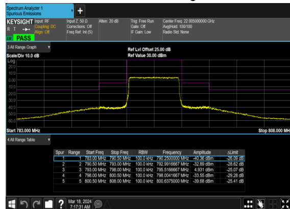
N14(5M)_CP-OFDM_16 QAM_Outer_Full_High_CH
