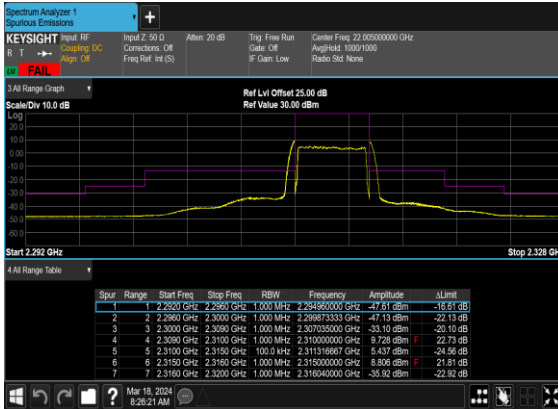
N30(5M)_DFT-s-OFDM_BPSK_Outer_Full_High_CH
