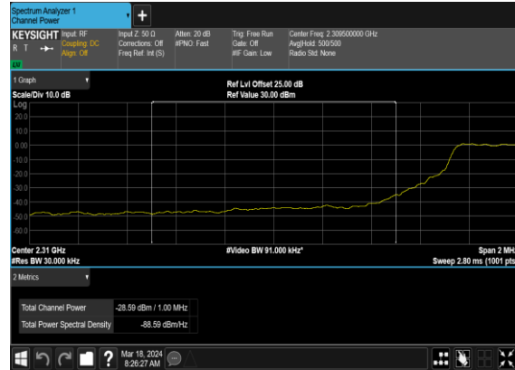
N30(5M)_DFT-s-OFDM_BPSK_Outer_Full_High_CH_CHP_PASS
