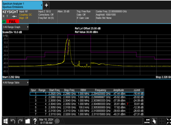
N30(5M)_DFT-s-OFDM_QPSK_Edge_1RB_Left_Low_CH
