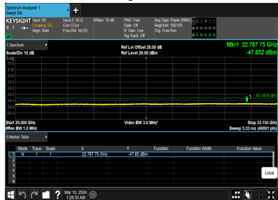
N30(5M)_DFT-s-OFDM_BPSK_Edge_1RB_Left_Mid_CH
