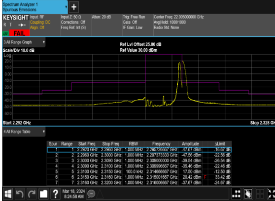
N30(5M)_DFT-s-OFDM_QPSK_Edge_1RB_Right_High_CH
