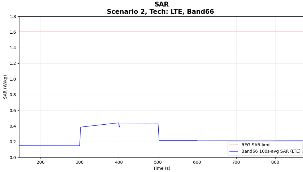
Figure 6-7 Time-averaged SAR
