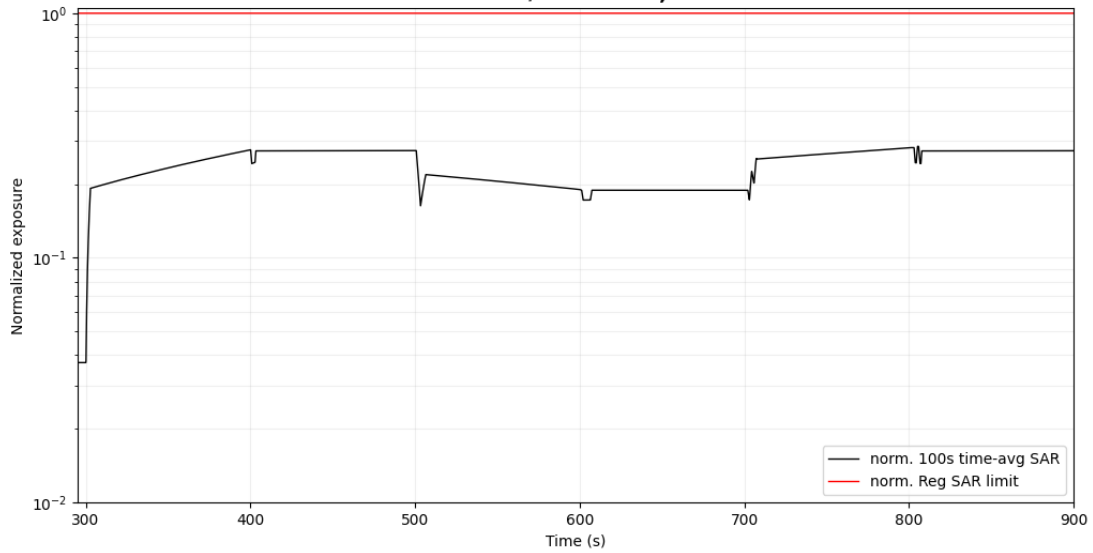
Total normalized Time-averaged RF exposure Scenario 5, Tech: LTE, ECI9 / Tech: LTE, ECI10
