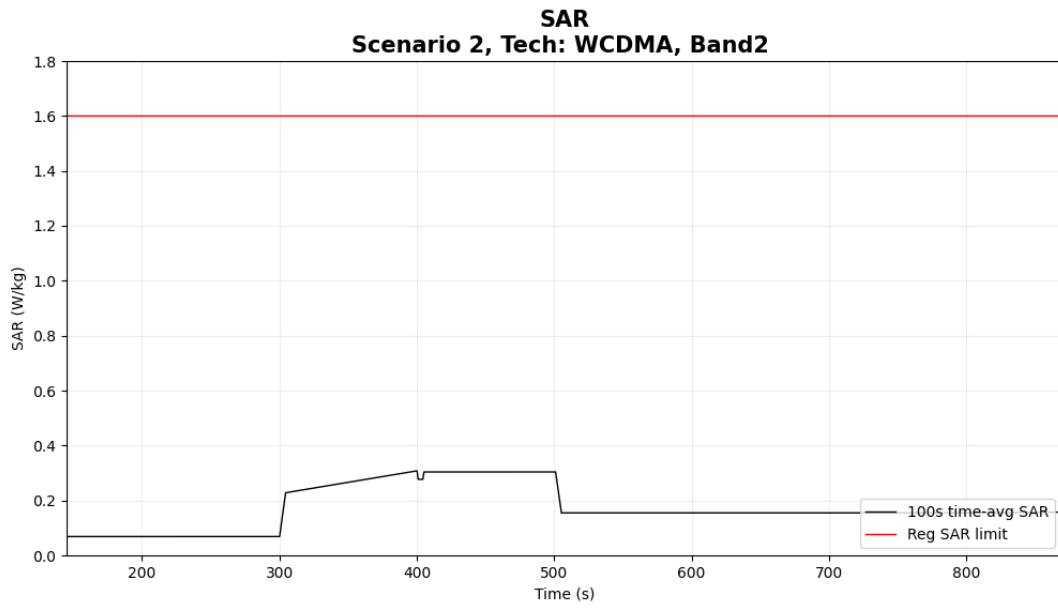
Figure 6- 16 Time-averaged SAR
