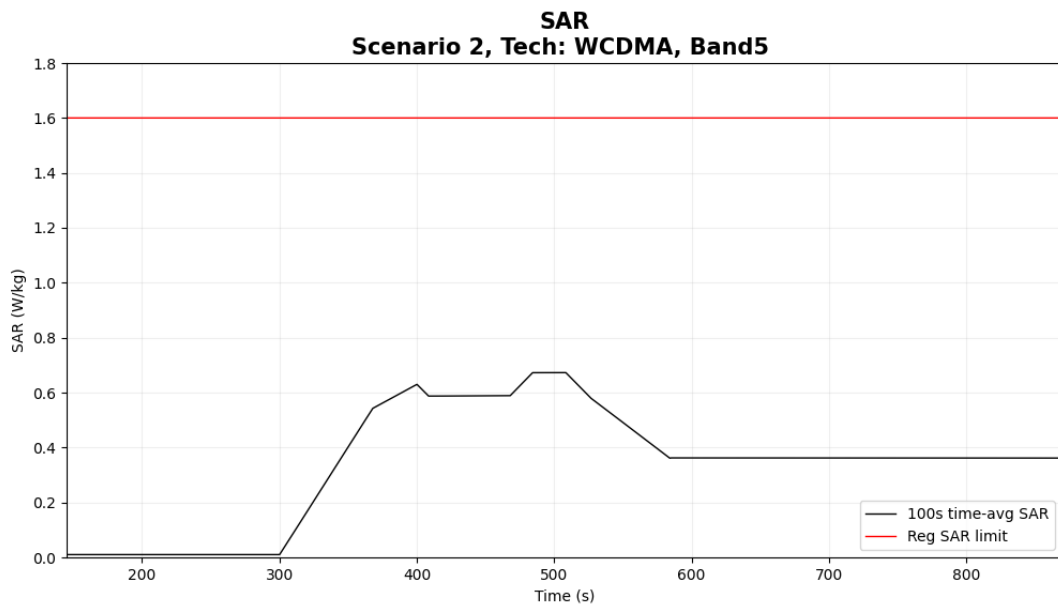
Figure 5- 19 Time-averaged SAR
