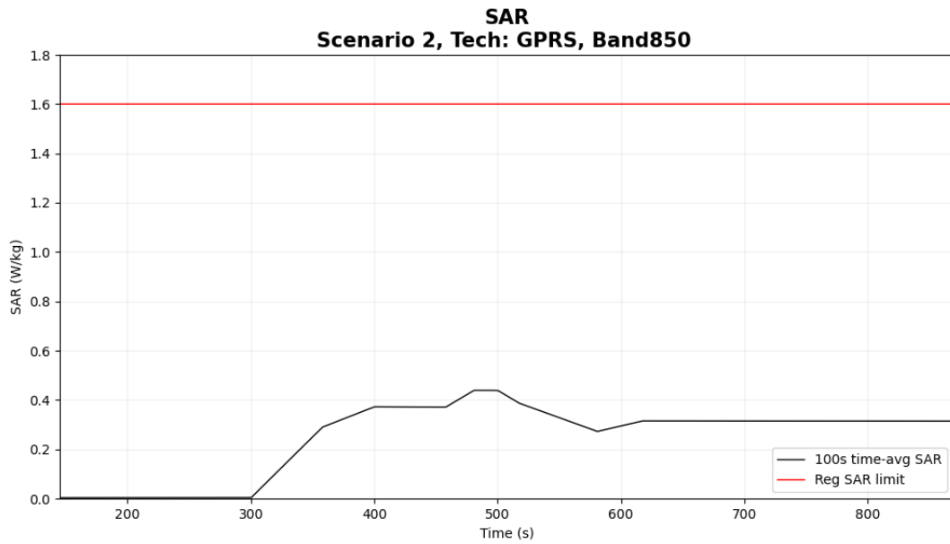
Figure 5- 8 Time-averaged SAR
