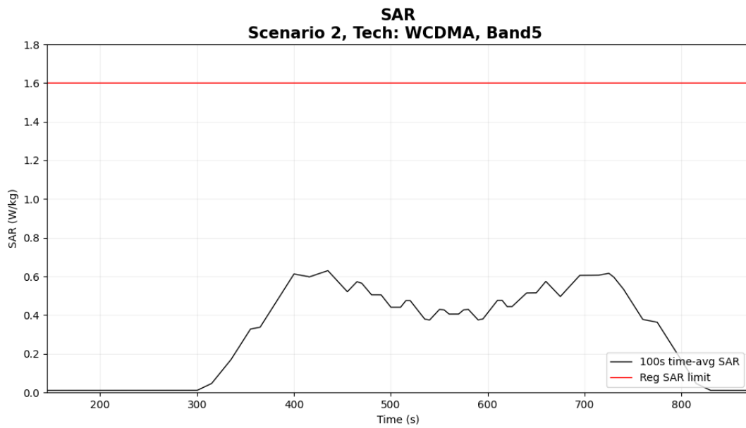
Figure 5- 21 Time-averaged SAR
