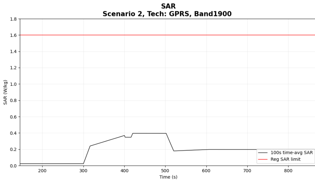
Figure 5- 12 Time-averaged SAR
