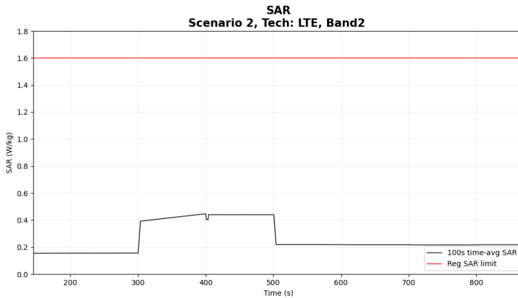
Figure 5- 23 Time-averaged SAR
