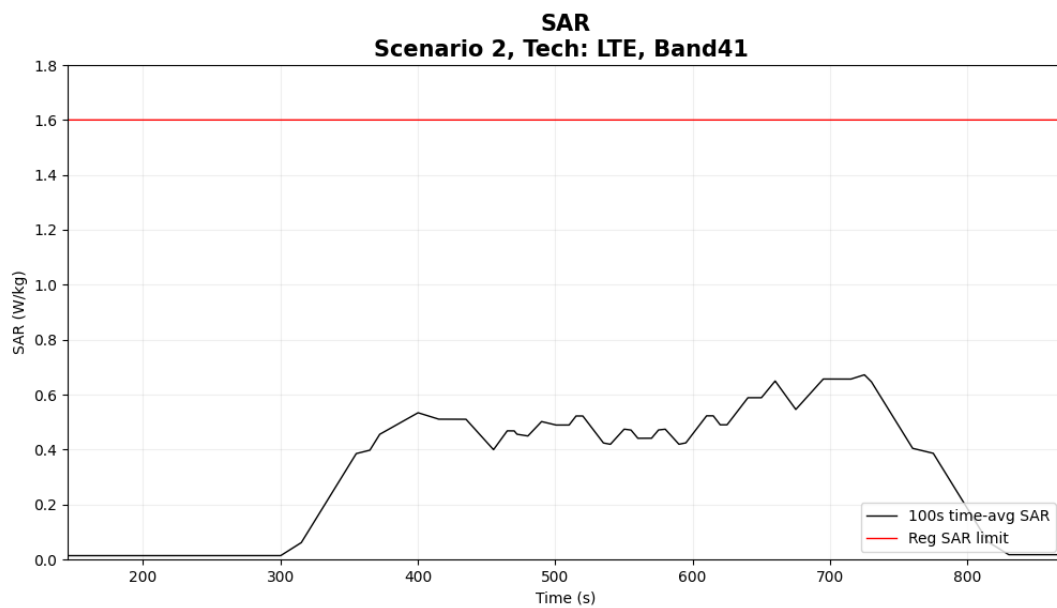
Figure 5- 28 Time-averaged SAR
