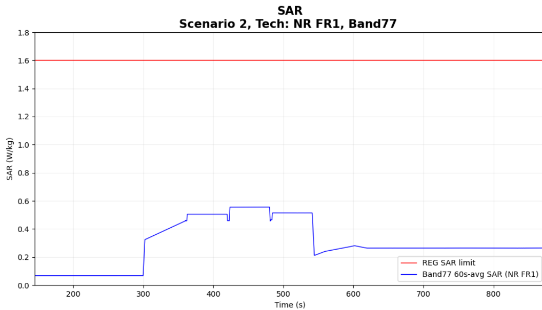
Figure 6-5 Time-averaged SAR
