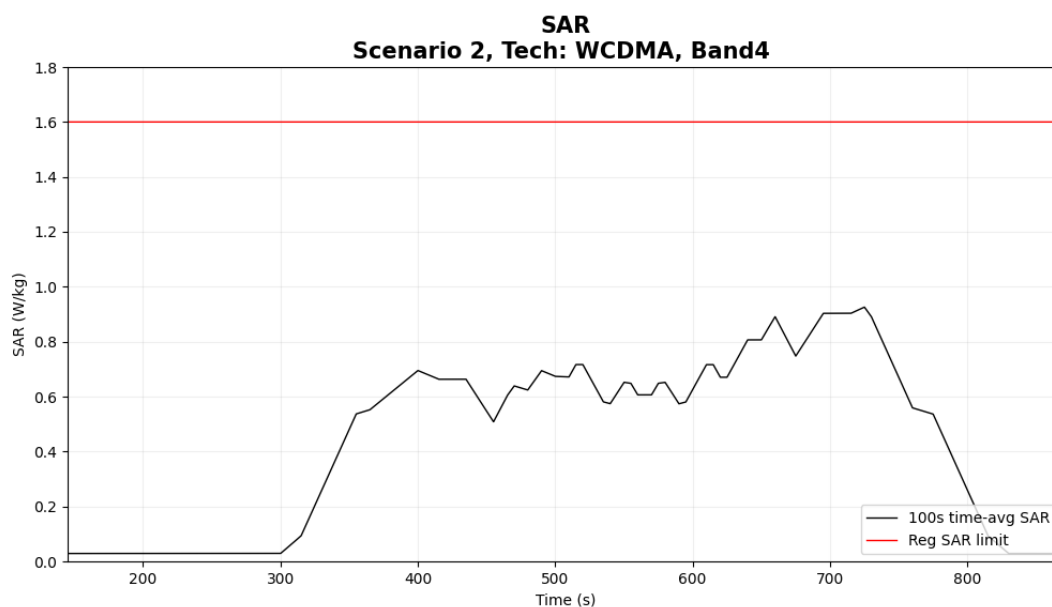
Figure 5- 21 Time-averaged SAR
