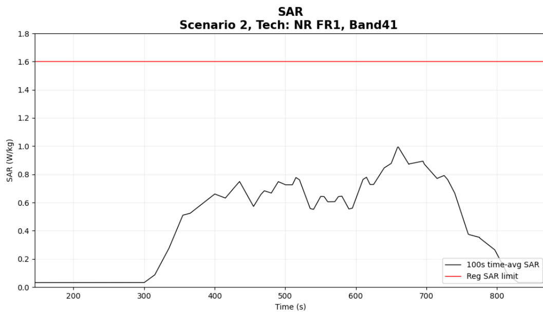
Figure 5- 36 Time-averaged SAR
