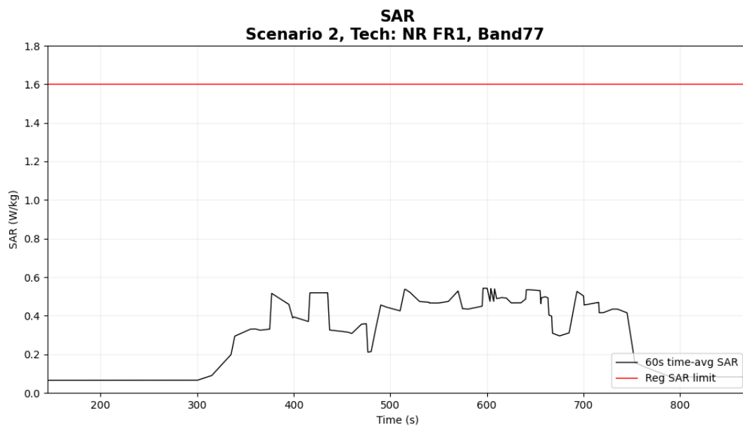
Figure 5- 32 Time-averaged SAR
