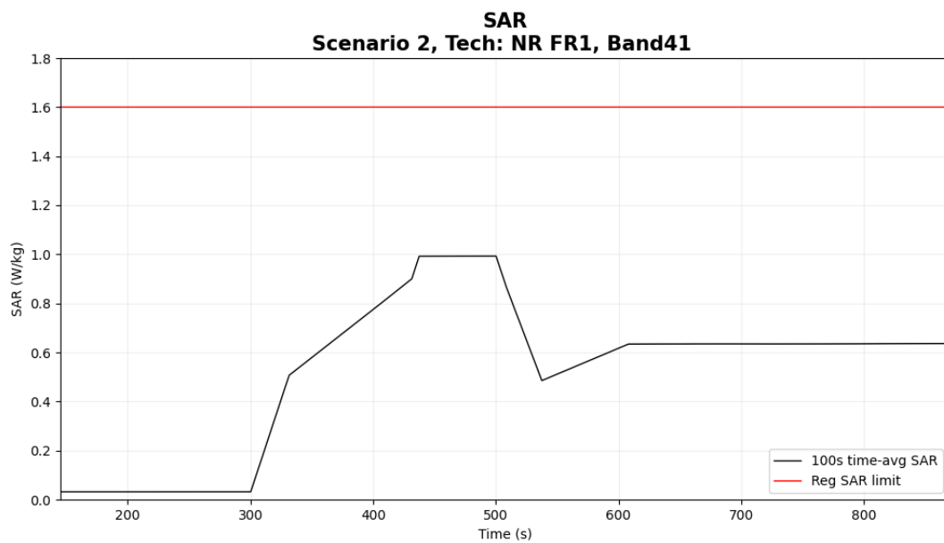
Figure 5- 34 Time-averaged SAR
