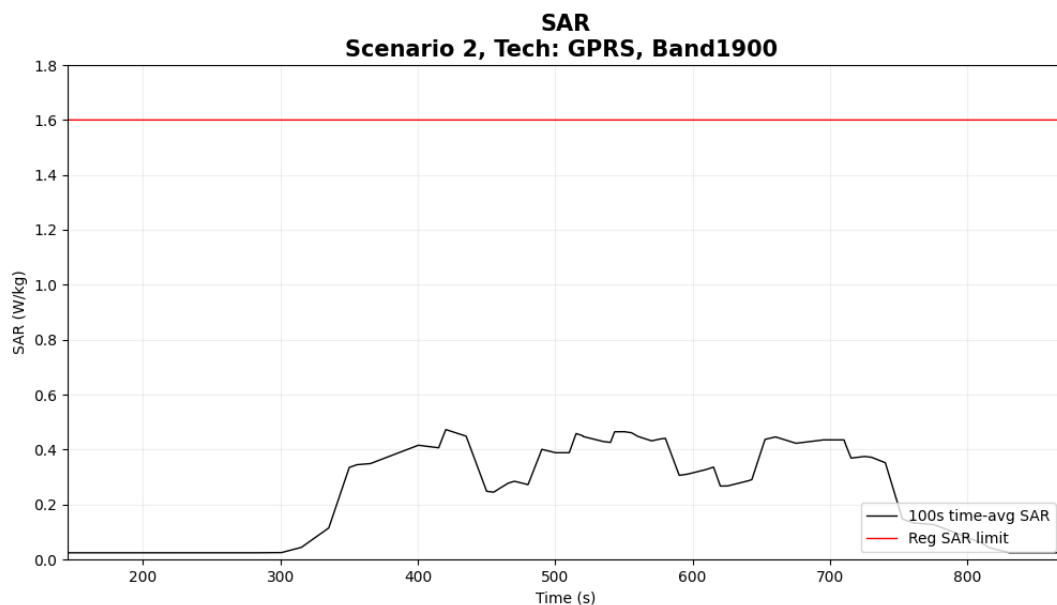
Figure 5- 14 Time-averaged SAR
