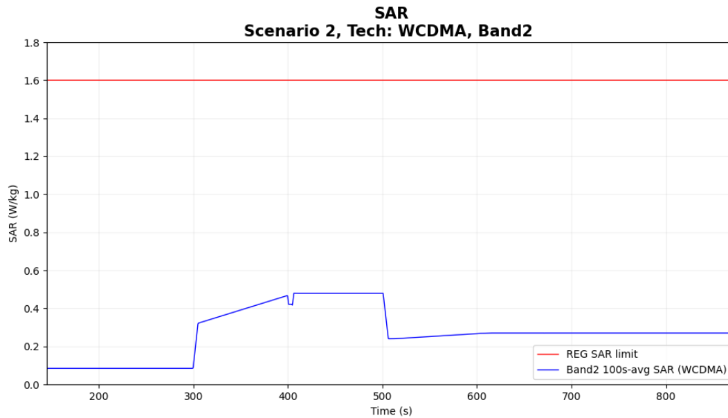
Figure 6-11 Time-averaged SAR
