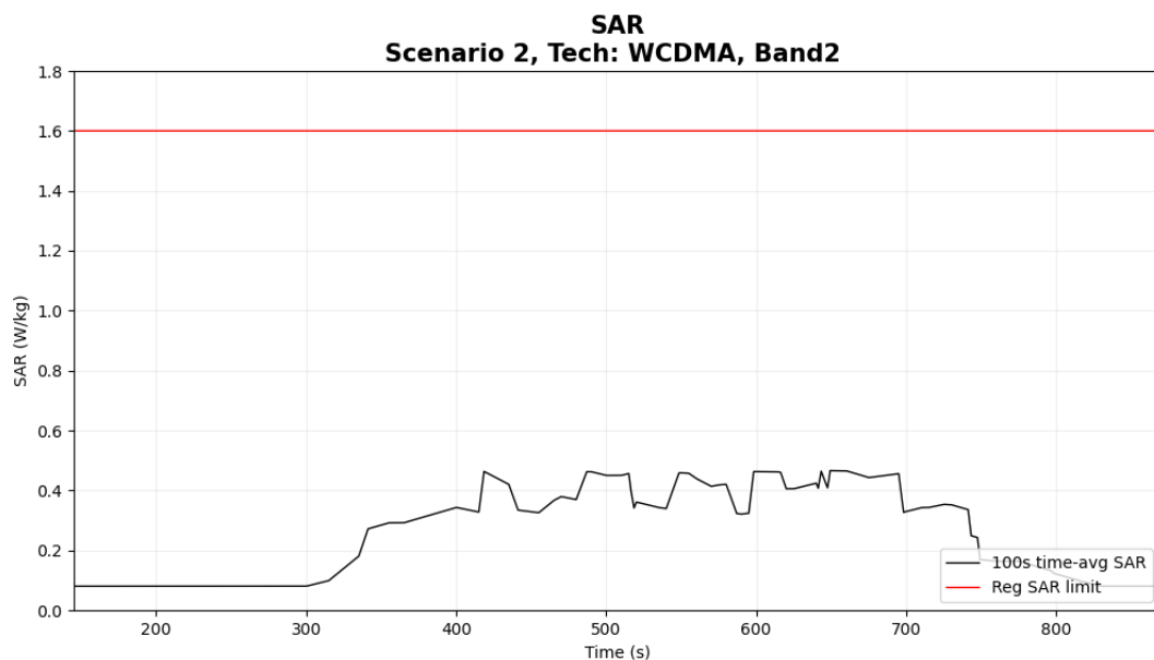
Figure 5- 17 Time-averaged SAR
