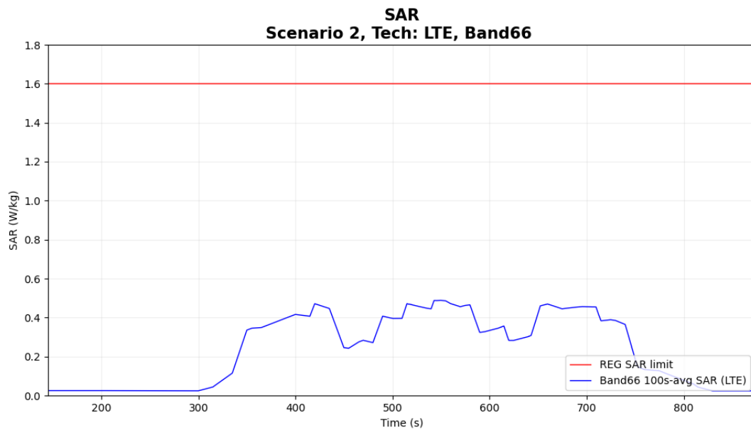
Figure 6-18 Time-averaged SAR
