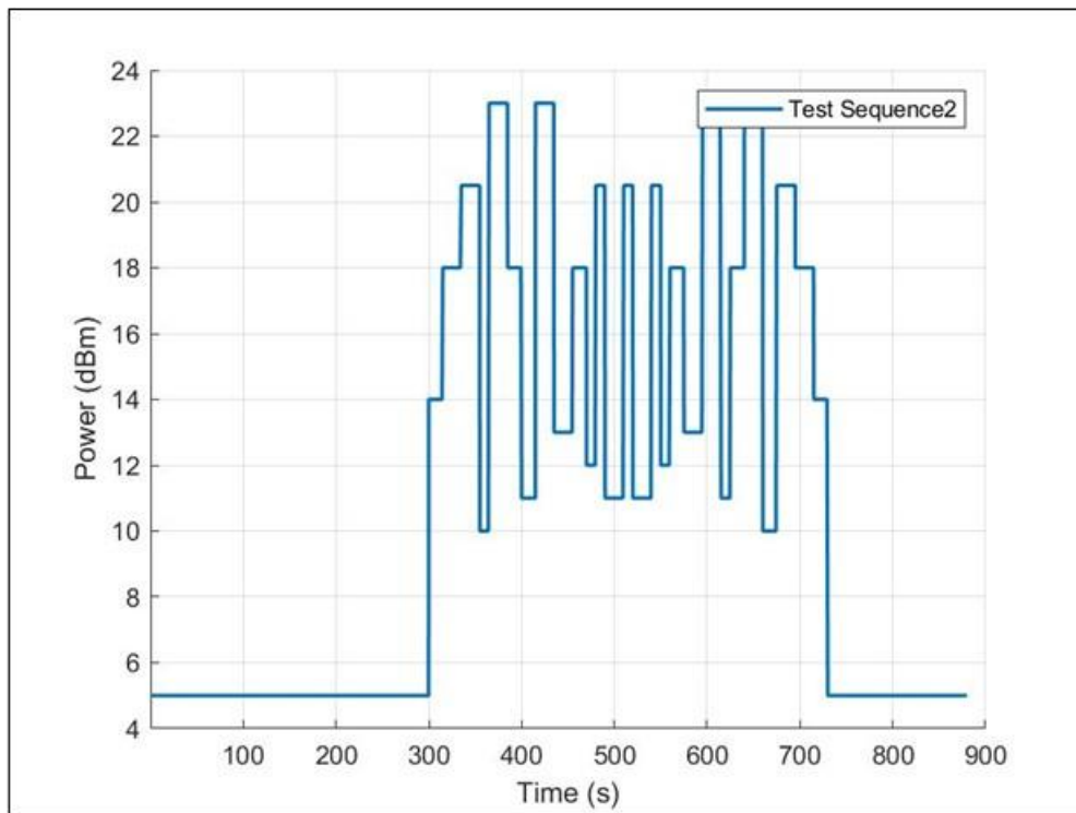
Figure 4-3 Test sequence 2
