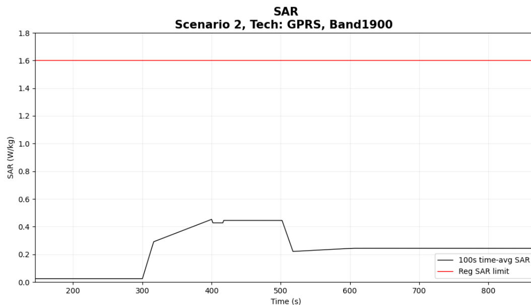
Figure 5- 12 Time-averaged SAR
