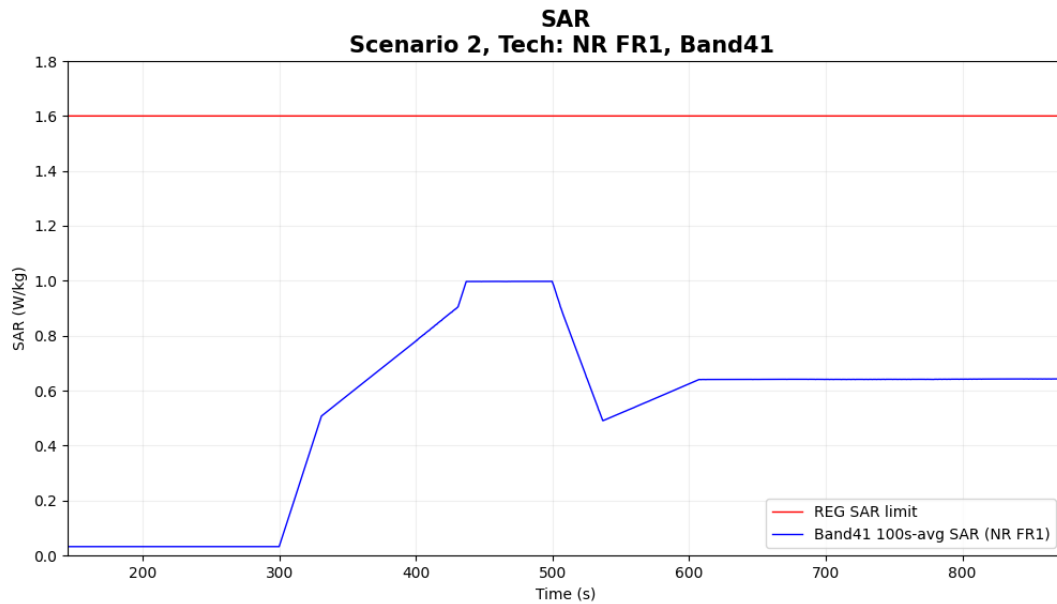
Figure 6-3 Time-averaged SAR
