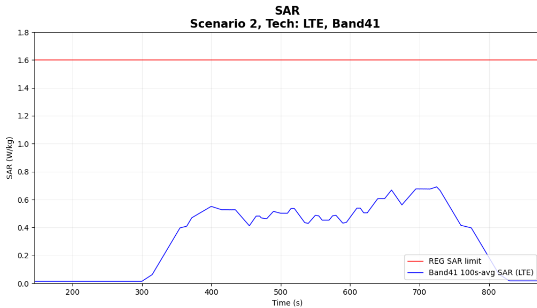
Figure 6-10 Time-averaged SAR
