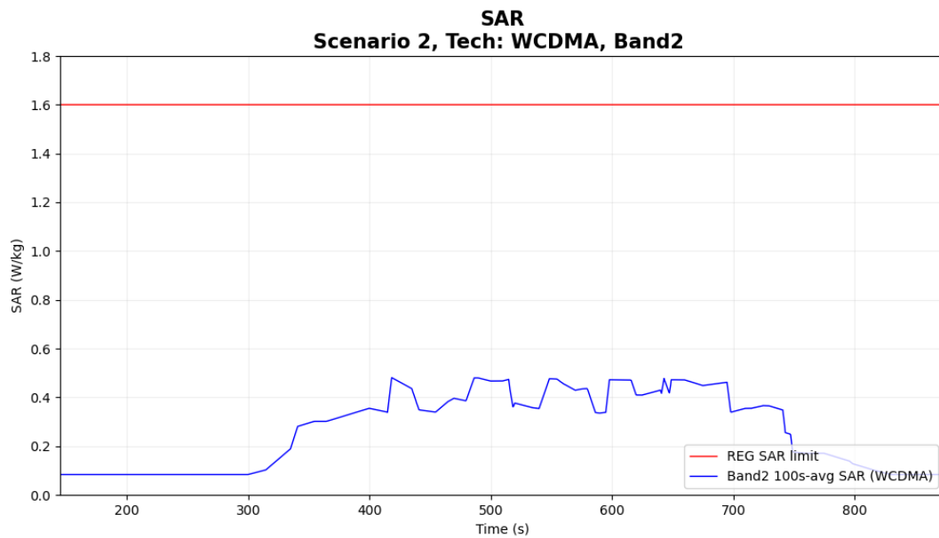
Figure 6-12 Time-averaged SAR
