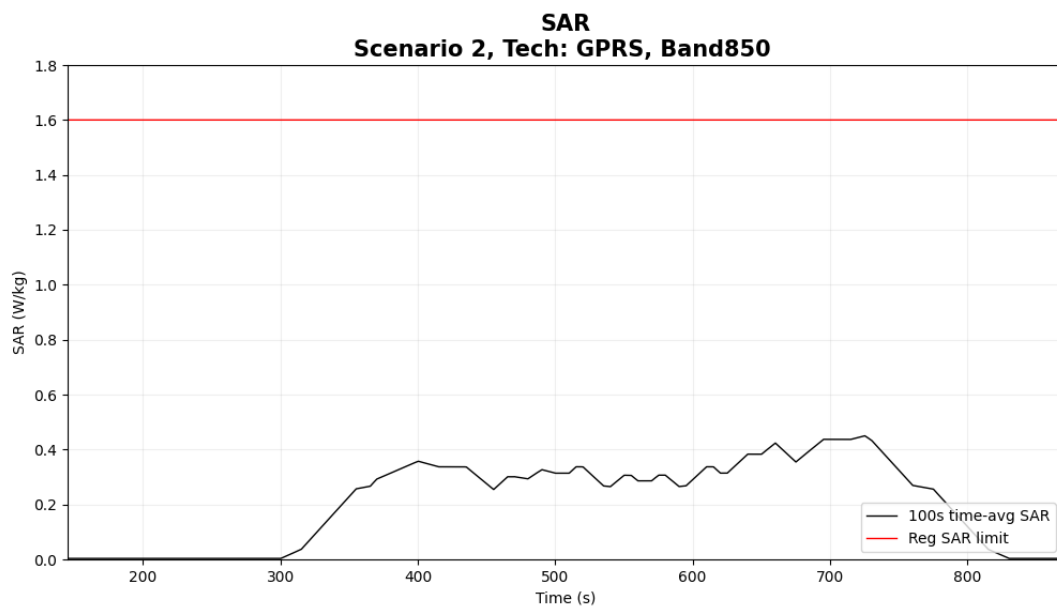
Figure 5- 10 Time-averaged SAR
