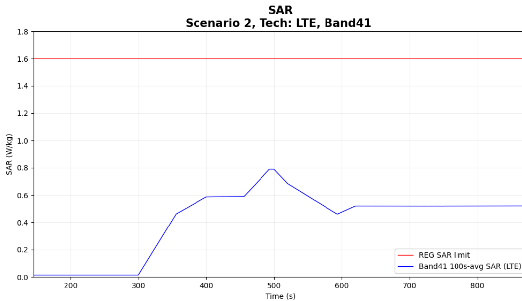
Figure 6-9 Time-averaged SAR
