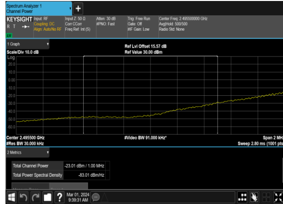
B4_N41(100M)_DFT-s- OFDM_QPSK_Edge_1RB_Left_Low_CH_chP PASS
