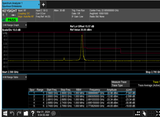
B4_N41(50M)_DFT-s-OFDM_BPSK_Edge_1RB_Right_High_CH
