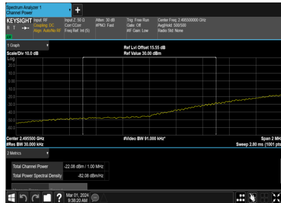
B4_N41(100M)_DFT-s-OFDM_BPSK_Edge_1RB_Left_Low_CH_chp_PASS
