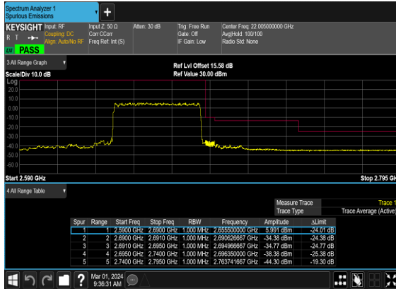
B4_N41(50M)_DFT-s-OFDM_BPSK_Outer_Full_High_CH
