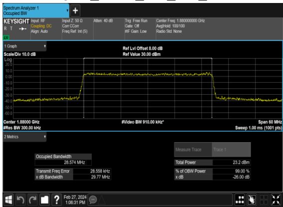
N2(30M)_CP-OFDM_256 QAM_Outer_Full_Mid_CH
