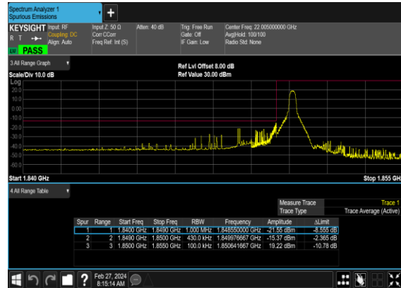
N2(40M)_DFT-s- OFDM_QPSK_Edge_1RB_Left_Low_CH
