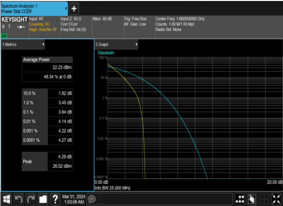
B4_N2(20M)_DFT-s-OFDM_PI_2-BPSK_Outer_Full_Mid_CH
