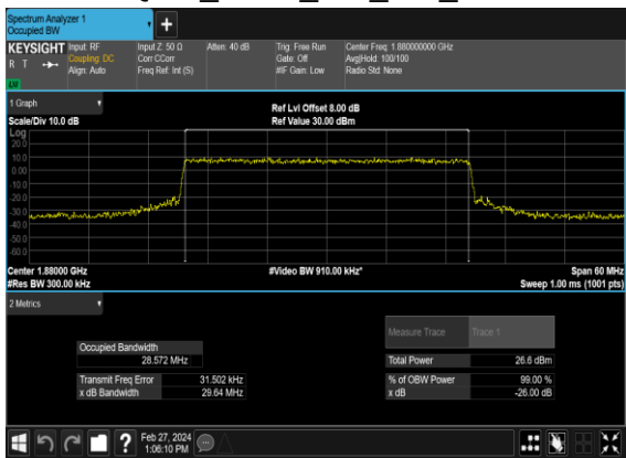
N2(30M)_CP-OFDM_16 QAM_Outer_Full_Mid_CH
