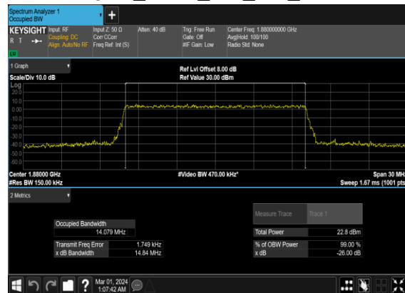
B4_N2(15M)_CP-OFDM_256 QAM_Outer_Full_Mid_CH
