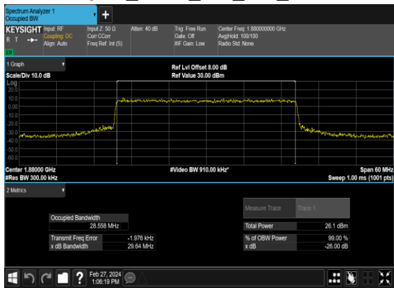
N2(30M)_CP-OFDM_64 QAM_Outer_Full_Mid_CH
