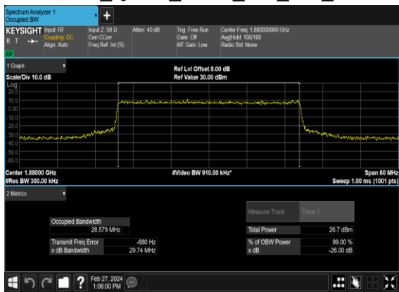
N2(30M)_CP- OFDM_QPSK_Outer_Full_Mid_CH
