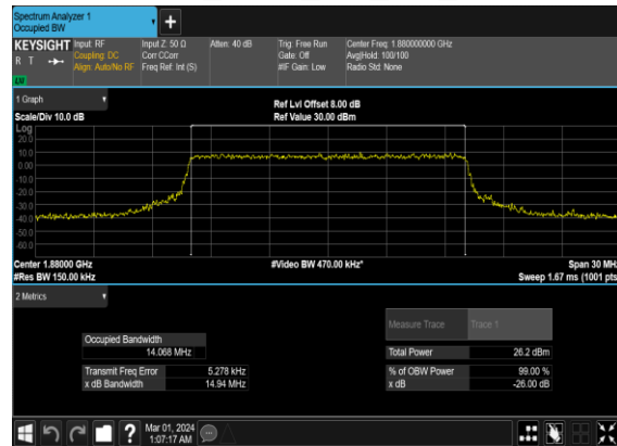
B4_N2(15M)_CP-OFDM_16 QAM_Outer_Full_Mid_CH
