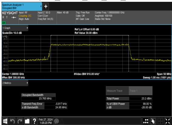
N2(25M)_CP-OFDM_256 QAM_Outer_Full_Mid_CH
