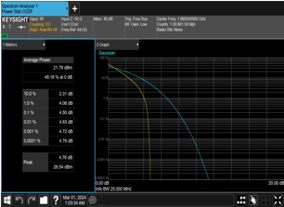
B4_N2(20M)_DFT-s-OFDM_QPSK_Outer_Full_Mid_CH
