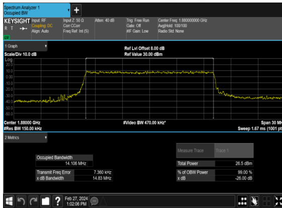
N2(15M)_CP- OFDM_QPSK_Outer_Full_Mid_CH
