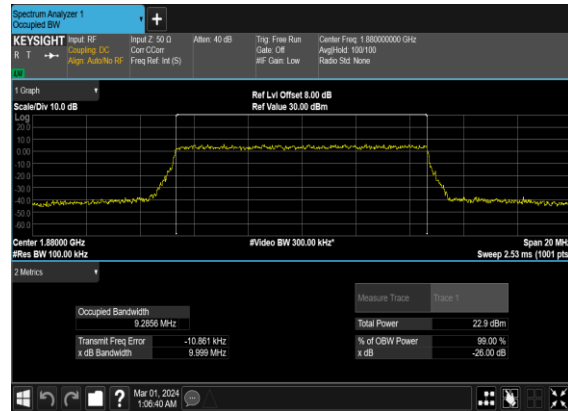
B4_N2(10M)_CP-OFDM_256 QAM_Outer_Full_Mid_CH
