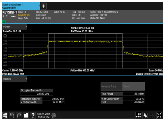
N2(25M)_CP-OFDM_64 QAM_Outer_Full_Mid_CH
