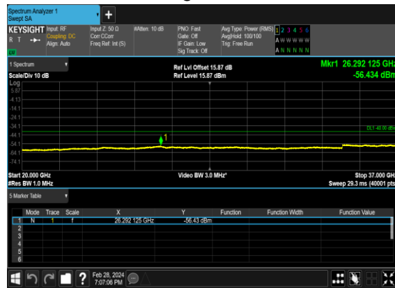
N48(20M)_DFT-s-OFDM_BPSK_Edge_1RB_Left_Mid_CH
