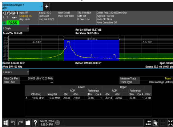
N48(10M)_DFT-s-OFDM_QPSK_Edge_1RB_Left_Mid_CH
