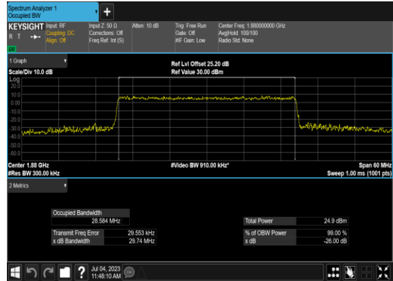
B7_N2(30M)_CP-OFDM_16 QAM_Outer_Full_Mid_CH
