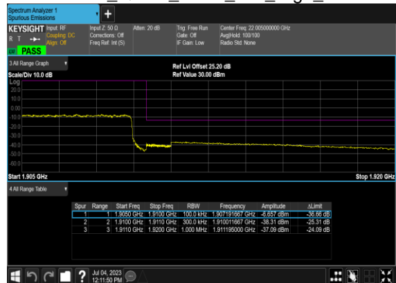
B7_N2(30M)_DFT-s-OFDM_QPSK_Outer_Full_High_CH
