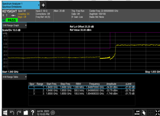
B7_N2(30M)_DFT-s-OFDM_BPSK_Outer_Full_Low_CH
