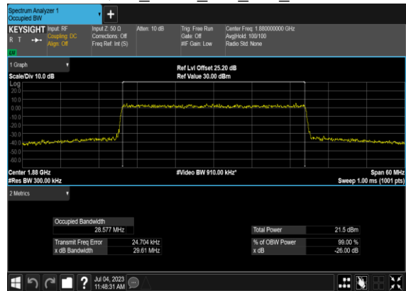
B7_N2(30M)_CP-OFDM_256 QAM_Outer_Full_Mid_CH
