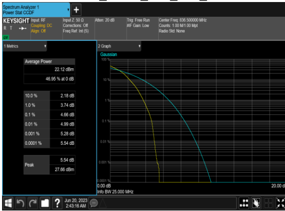
N5(25M)_DFT-s-OFDM_PI_2-BPSK_Outer_Full_Mid_CH
