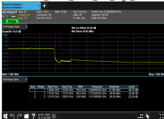
B7_N2(30M)_DFT-s-OFDM_BPSK_Outer_Full_High_CH
