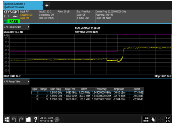
B7_N2(30M)_DFT-s-OFDM_QPSK_Outer_Full_Low_CH
