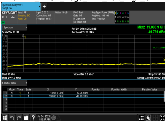
B7_N2(5M)_DFT-s-OFDM_BPSK_Edge_1RB_Left_High_CH
