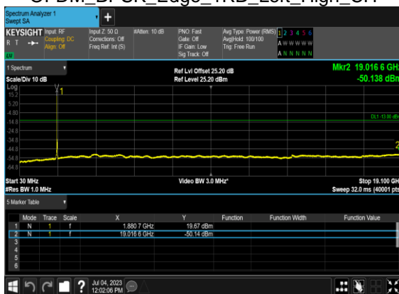
B7_N2(30M)_DFT-s-OFDM_BPSK_Edge_1RB_Left_High_CH
