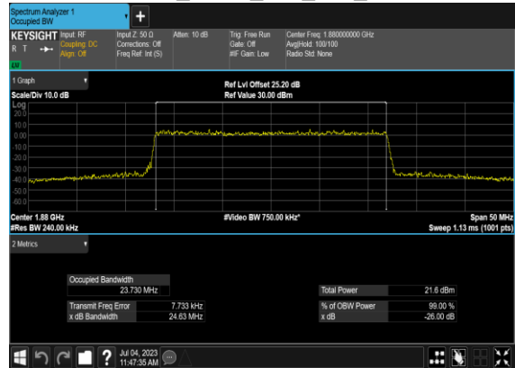
B7_N2(25M)_CP-OFDM_256 QAM_Outer_Full_Mid_CH
