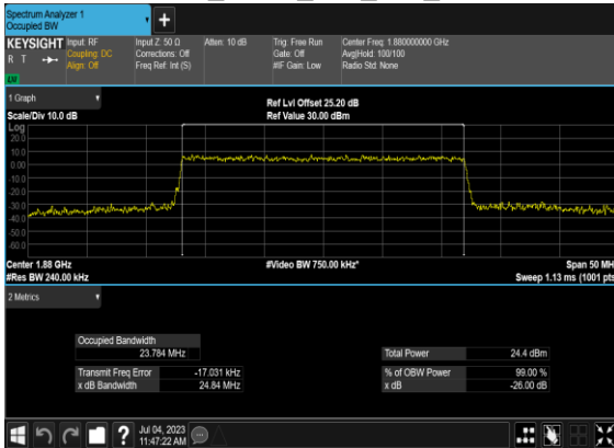
B7_N2(25M)_CP-OFDM_64 QAM_Outer_Full_Mid_CH
