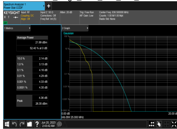
N5(25M)_DFT-s-OFDM_PI_2-BPSK_Edge_1RB_Left_Mid_CH
