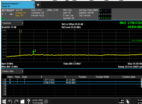
B7_N2(5M)_DFT-s-OFDM_BPSK_Edge_1RB_Left_Mid_CH
