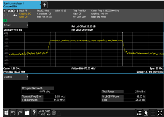
B7_N2(15M)_CP-OFDM_16 QAM_Outer_Full_Mid_CH
