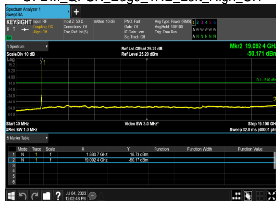
B7_N2(30M)_DFT-s-OFDM_QPSK_Edge_1RB_Left_High_CH
