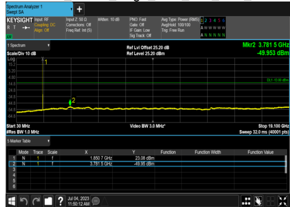
B7_N2(5M)_DFT-s-OFDM_QPSK_Edge_1RB_Left_Low_CH
