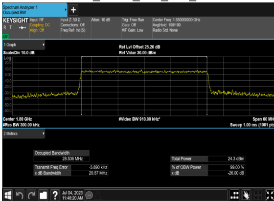
B7_N2(30M)_CP-OFDM_64 QAM_Outer_Full_Mid_CH
