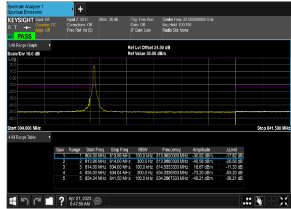
N26(20M)_DFT-s-OFDM_QPSK_Edge_1RB_Right_
