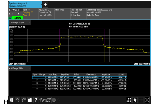
N26(5M)_DFT-s-OFDM_QPSK_Outer_Full_High_C
