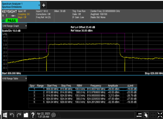
N26(10M)_DFT-s-OFDM_BPSK_Outer_Full_Mid_C
