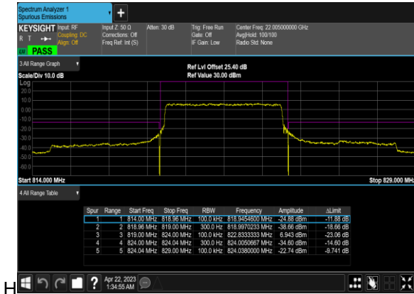
N26(5M)_DFT-s-OFDM_BPSK_Outer_Full_High_C
