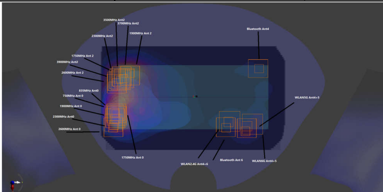
WWAN+WLAN+BT_Front 5mm
