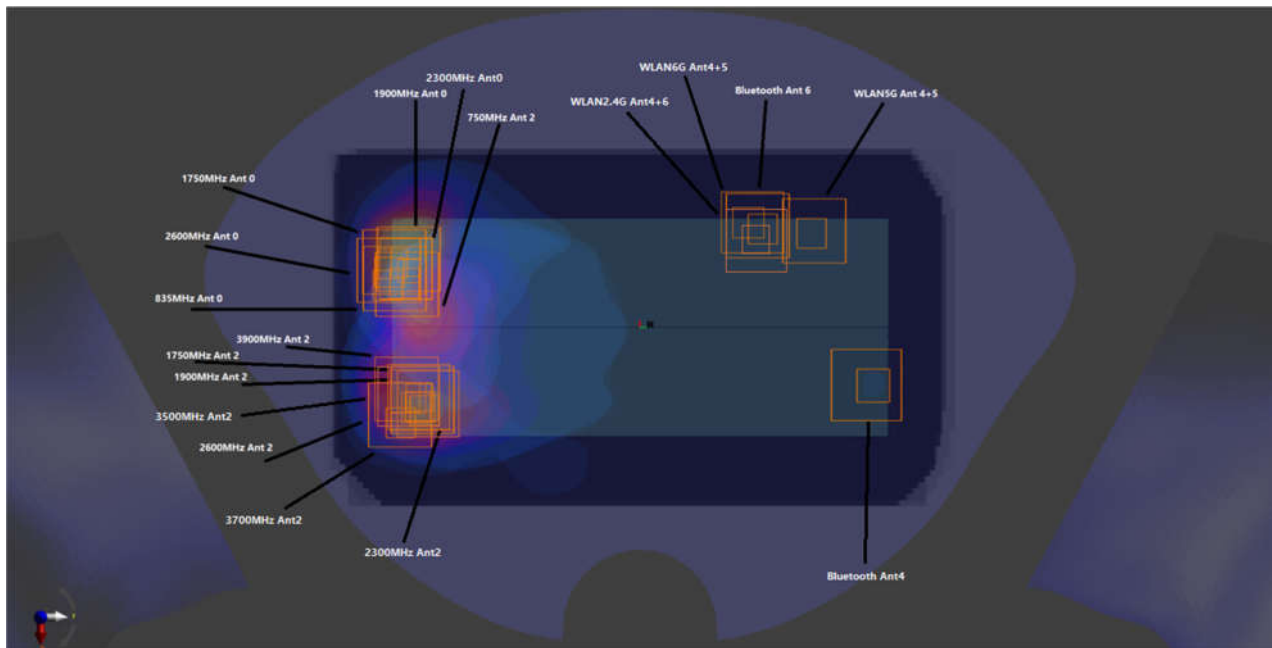
WWAN+WLAN+BT_Back 5mm
