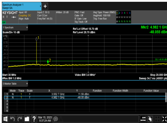
N48(10M)_DFT-s-OFDM_QPSK_Outer_Full_Low_CH
