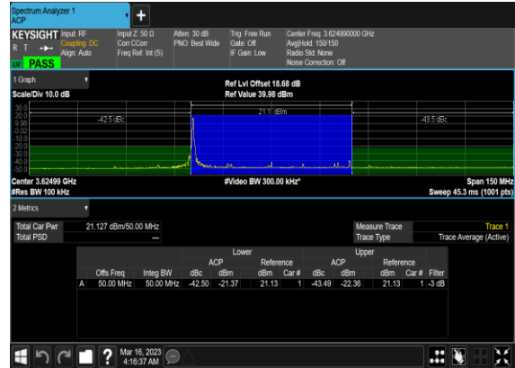
N48(50M)_DFT-s-OFDM_PI_2-BPSK_Edge_1RB_Left_Mid_CH
