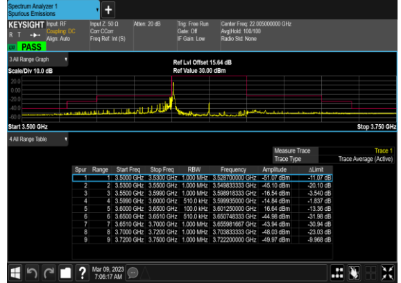
N48(50M)_DFT-s-OFDM_QPSK_Edge_1RB_Left_Mid_CH
