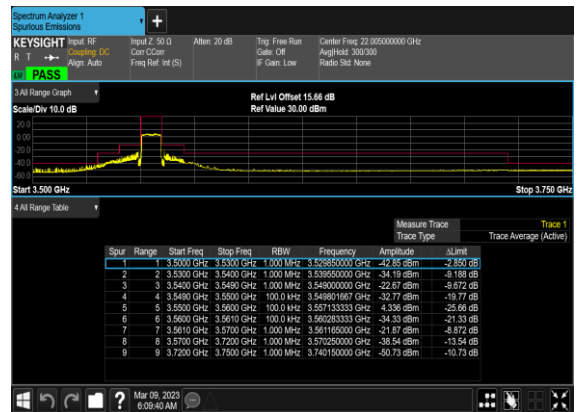
N48(10M)_DFT-s-OFDM_QPSK_Outer_Full_Low_CH
