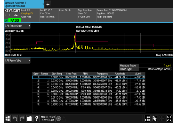
N48(50M)_DFT-s-OFDM_QPSK_Edge_1RB_Right_Low_CH
