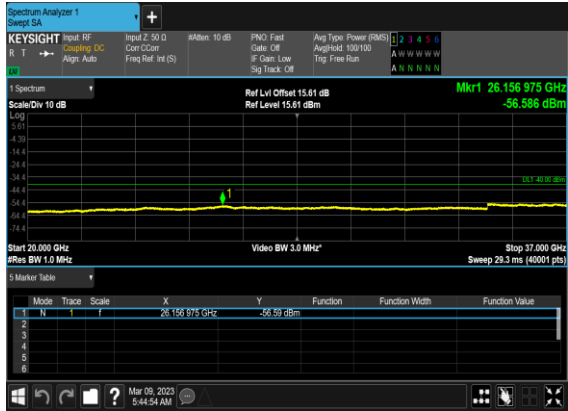
N48(100M)_DFT-s-OFDM_QPSK_Edge_1RB_Right_Mid_CH
