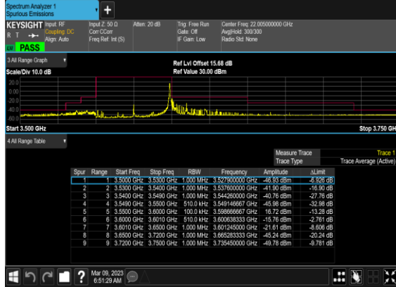
N48(50M)_DFT-s-OFDM_BPSK_Edge_1RB_Right_Low_CH
