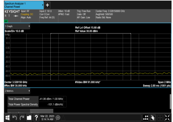
N48(50M)_DFT-s-OFDM_BPSK_Outer_Full_Low_CH_CHP_PASS
