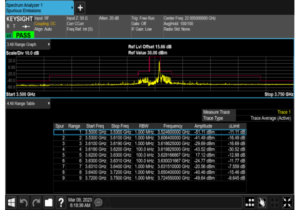
N48(10M)_DFT-s-OFDM_QPSK_Edge_1RB_Right_Mid_CH
