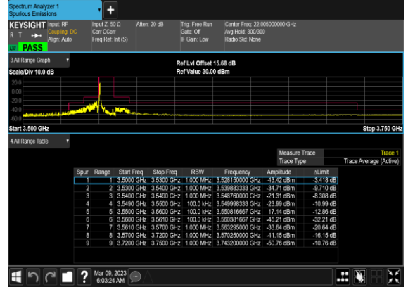
N48(10M)_DFT-s-OFDM_QPSK_Edge_1RB_Left_Low_CH
