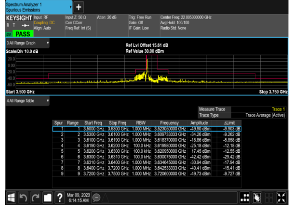
N48(10M)_DFT-s-OFDM_QPSK_Edge_1RB_Left_Mid_CH
