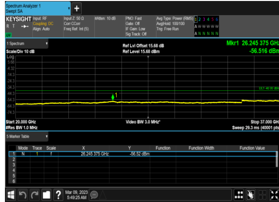
N48(100M)_DFT-s-OFDM_BPSK_Edge_1RB_Left_High_CH
