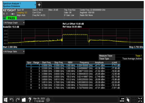
N48(50M)_DFT-s-OFDM_QPSK_Outer_Full_Mid_CH
