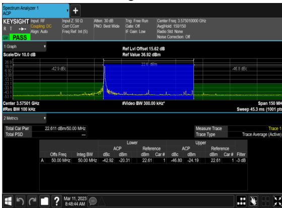
N48(50M)_DFT-s-OFDM_QPSK_Edge_1RB_Left_Low_CH
