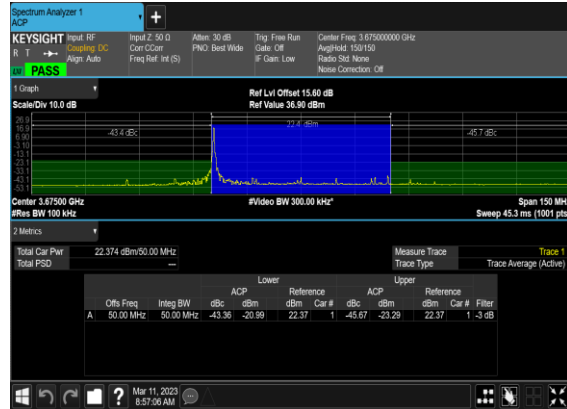
N48(50M)_DFT-s-OFDM_PI_2-BPSK_Edge_1RB_Left_High_CH
