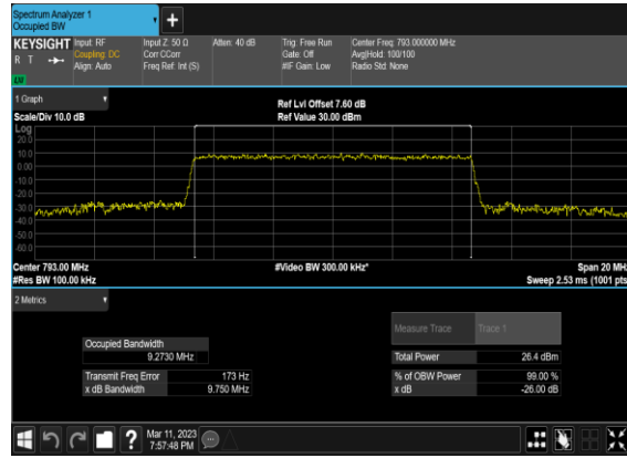
N14(10M)_CP-OFDM_16QAM_Outer_Full_Mid_CH
