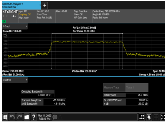
N14(5M)_CP- OFDM_QPSK_Outer_Full_Mid_CH
