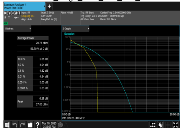
N77(20M)_DFT-s-OFDM_PI_2-BPSK_Edge_1RB_Left_Mid_CH
