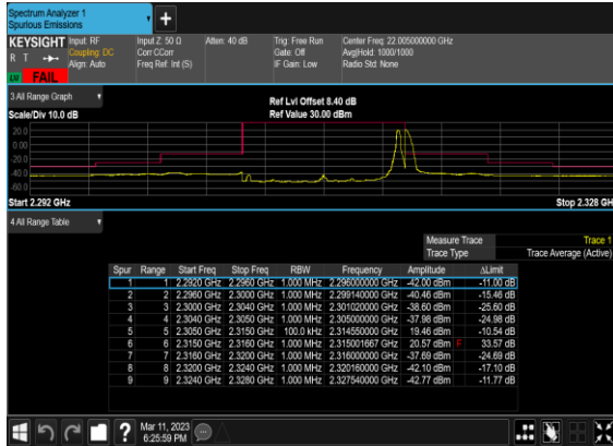
N30(10M)_DFT-s- OFDM_BPSK_Edge_1RB_Right_Low_CH
