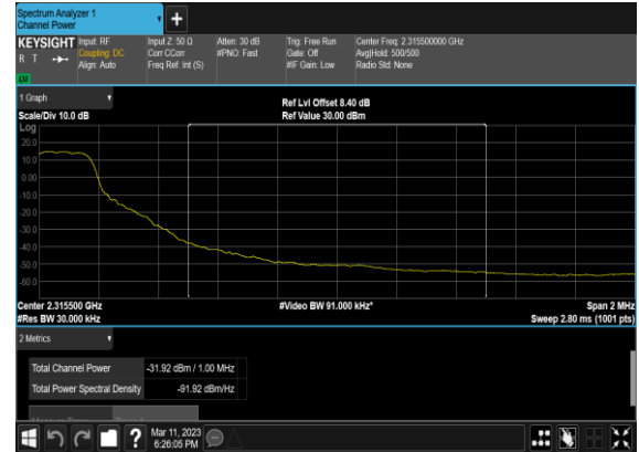
N30(10M)_DFT-s- OFDM_BPSK_Edge_1RB_Right_Low_CH_CHP_PASS
