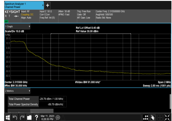
N30(10M)_DFT-s- OFDM_QPSK_Edge_1RB_Right_Low_CH_CHP_PASS
