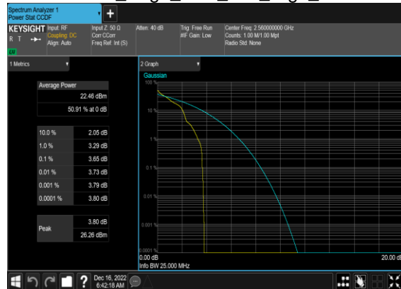
N7(20M)_DFT-s-OFDM_PI_2-BPSK_Edge_1RB_Left_High_CH
