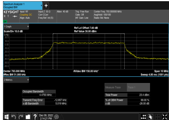
N14(5M)_CP-OFDM_256 QAM_Outer_Full_Mid_CH
