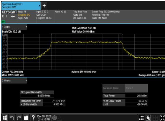
N14(5M)_CP-OFDM_64 QAM_Outer_Full_Mid_CH
