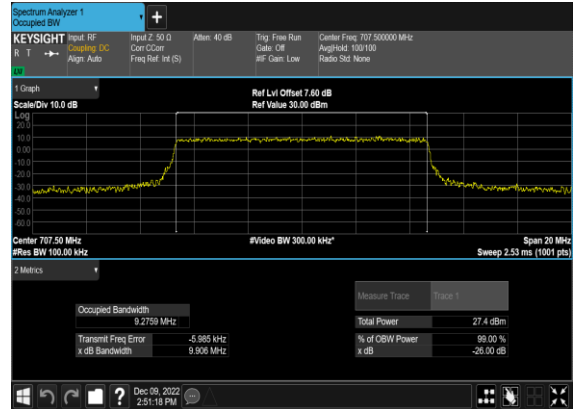
N12(10M)_CP-OFDM_16 QAM_Outer_Full_Mid_CH
