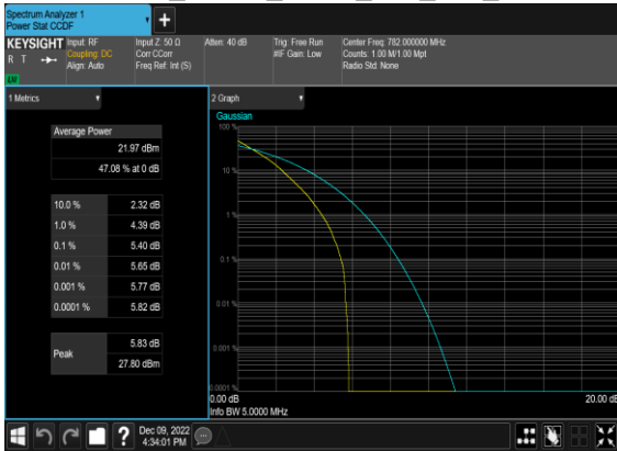
N13(5M)_DFT-s-OFDM_QPSK_Outer_Full_Mid_CH
