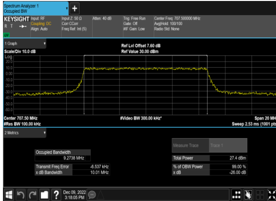
N12(10M)_CP- OFDM_QPSK_Outer_Full_Mid_CH
