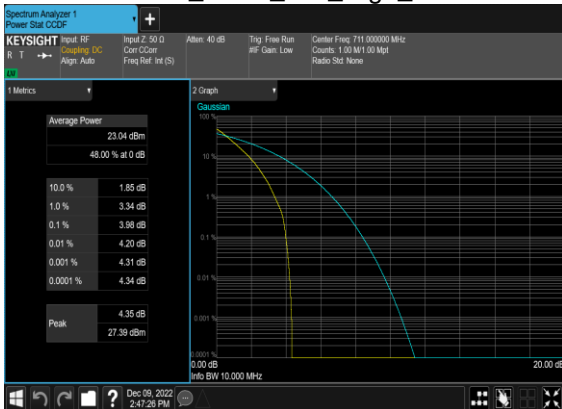
N12(10M)_DFT-s-OFDM_PI_2-BPSK_Outer_Full_High_CH
