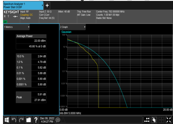
N13(5M)_DFT-s-OFDM_QPSK_Edge_1RB_Left_Mid_CH
