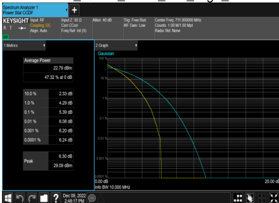
N12(10M)_DFT-s-OFDM_QPSK_Outer_Full_High_CH
