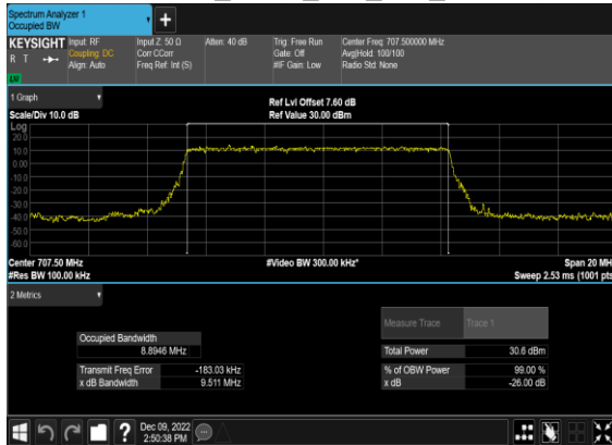
N12(10M)_DFT-s-OFDM_PI_2- BPSK_Outer_Full_Mid_CH
