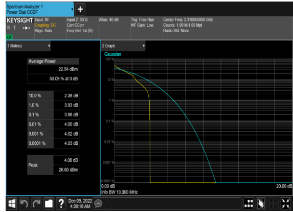
N30(10M)_DFT-s-OFDM_QPSK_Edge_1RB_Left_Low_CH
