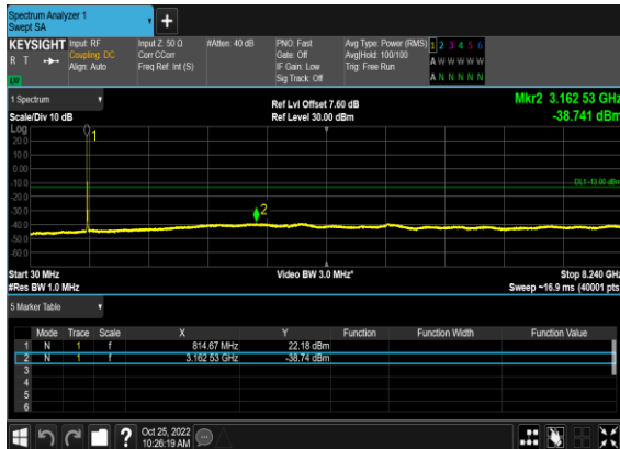
N26(20M)_DFT-s-OFDM_BPSK_Edge_1RB_Left_Mi
