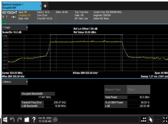
N26(20M)_DFT-s-OFDM_PI_2-BPSK_Outer_Full_Mid_
