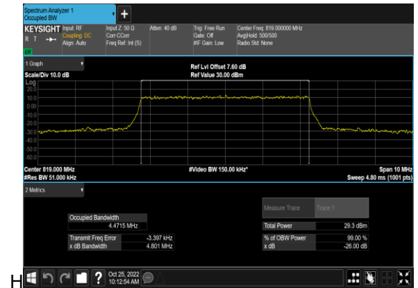
N26(5M)_DFT-s-OFDM_QPSK_Outer_Full_Mid_C
