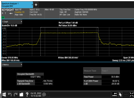
N26(10M)_DFT-s-OFDM_PI_2-BPSK_Outer_Full_Mid_
