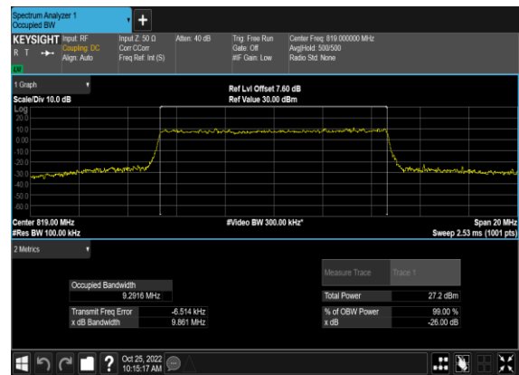
QAM_Outer_Full_Mid_CH
