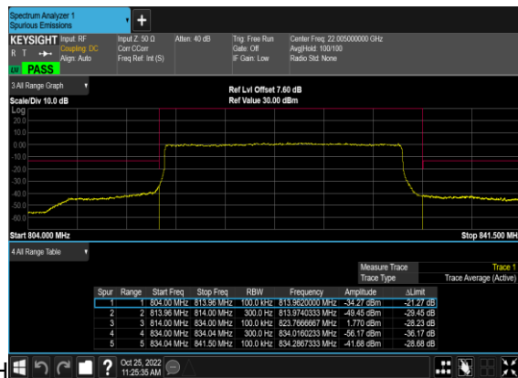
N26(20M)_DFT-s-OFDM_BPSK_Outer_Full_Low_C
