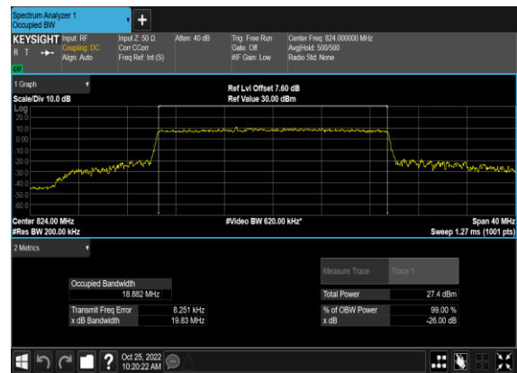
N26(20M)_CP-OFDM_16 QAM_Outer_Full_Mid_CH
