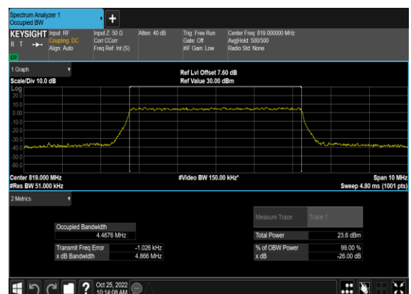
N26(5M)_CP-OFDM_256 QAM_Outer_Full_Mid_CH
