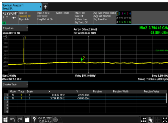
N26(20M)_DFT-s-OFDM_BPSK_Edge_1RB_Left_Mi
