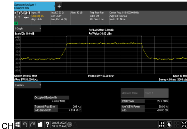
N26(5M)_DFT-s-OFDM_PI_2-BPSK_Outer_Full_Mid_
