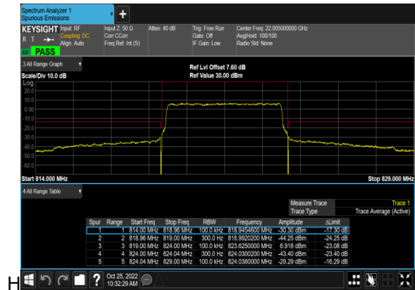
N26(5M)_DFT-s-OFDM_QPSK_Outer_Full_High_C
