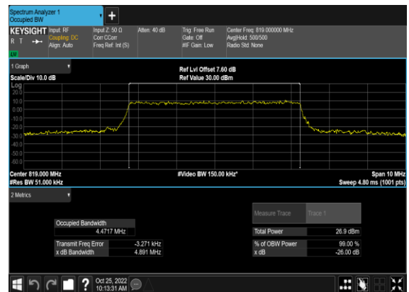
N26(5M)_CP-OFDM_16 QAM_Outer_Full_Mid_CH
