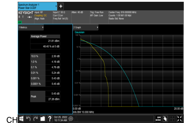
N26(10M)_DFT-s-OFDM_QPSK_Edge_1RB_Left_Mid_CH
