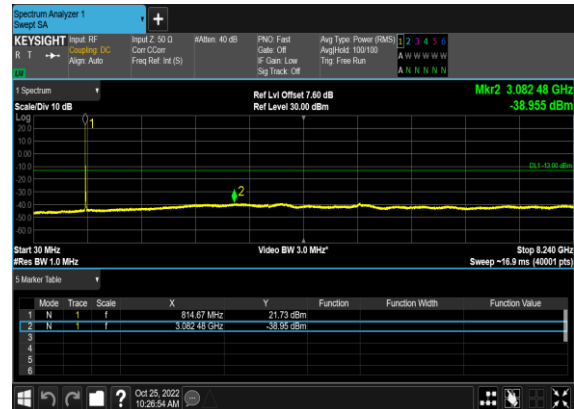
N26(20M)_DFT-s-OFDM_QPSK_Edge_1RB_Left_Mi
