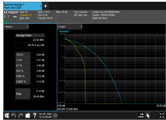
N26(10M)_DFT-s-OFDM_PI_2-BPSK_Edge_1RB_Left_Mid_CH
