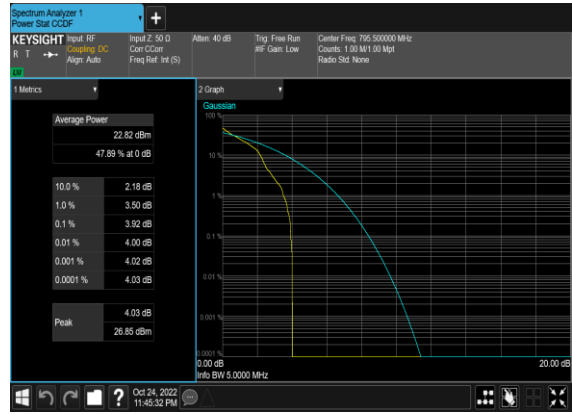
N14(5M)_DFT-s-OFDM_PI_2-BPSK_Edge_1RB_Left_High_CH
