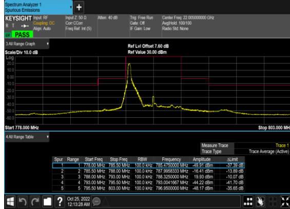
N14(5M)_DFT-s- OFDM_QPSK_Edge_1RB_Left_Low_CH
