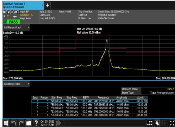
N14(5M)_DFT-s- OFDM_QPSK_Edge_1RB_Right_Low_CH
