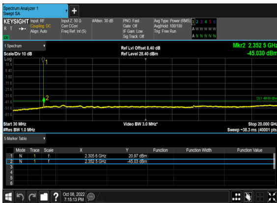
N30(10M)_DFT-s-OFDM_QPSK_Edge_1RB_Left_L ow_CH
