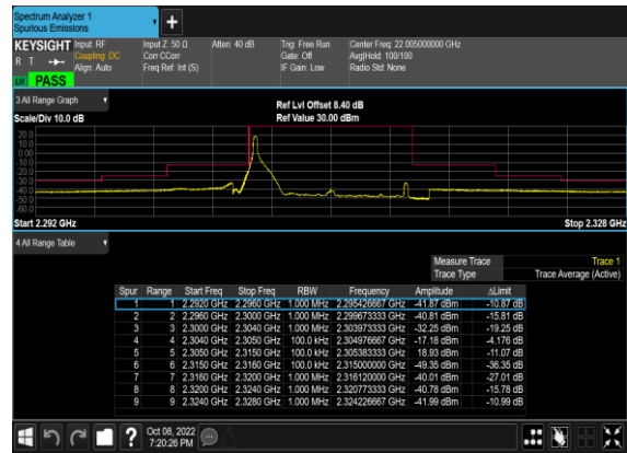
N30(10M)_DFT-s-OFDM_QPSK_Edge_1RB_Right_L
