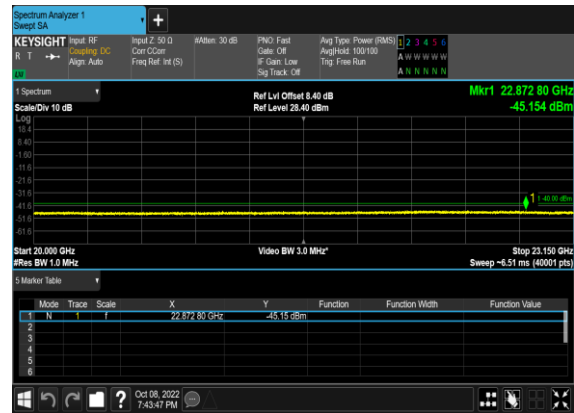
N30(5M)_DFT-s-OFDM_QPSK_Edge_1RB_Left_Lo
