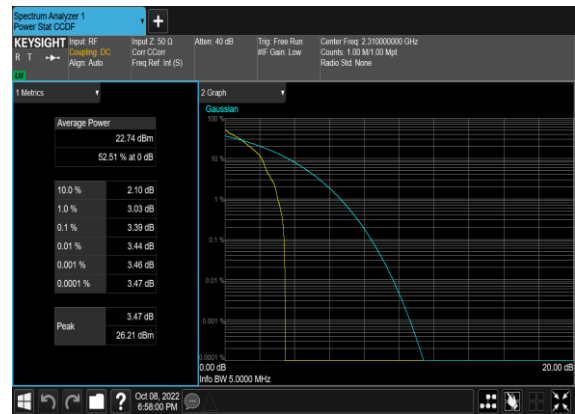
N30(5M)_DFT-s-OFDM_PI_2-BPSK_Edge_1RB_Left_Mid_CH
