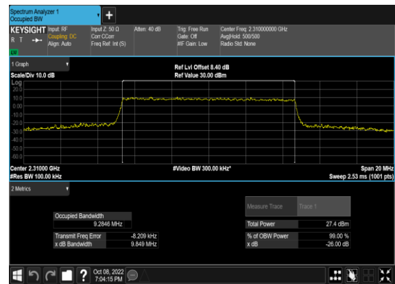
N30(10M)_CP-OFDM_16 QAM_Outer_Full_Low_CH
