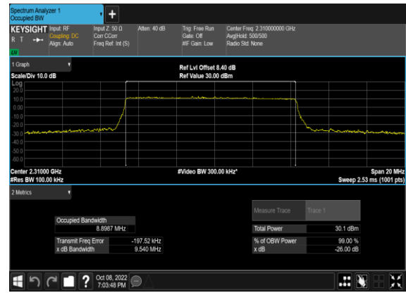
N30(10M)_DFT-s-OFDM_QPSK_Outer_Full_Low_CH
