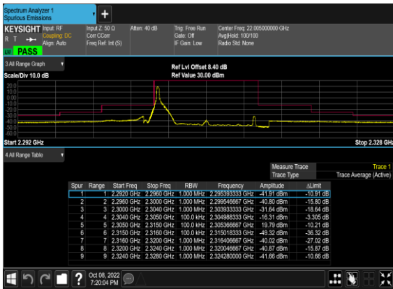
N30(10M)_DFT-s-OFDM_BPSK_Edge_1RB_Right_L
