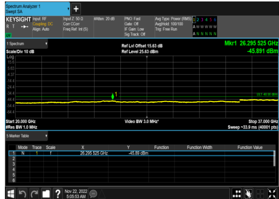
N48(10M)_DFT-s-OFDM_BPSK_Edge_1RB_Left_High_CH
