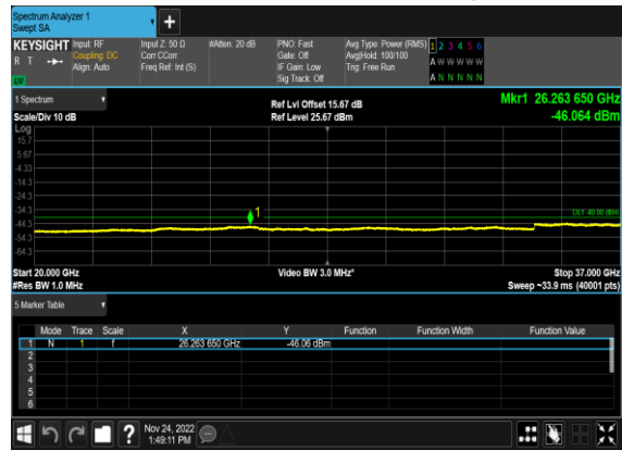
N48(20M)_DFT-s-OFDM_BPSK_Outer_Full_High_CH
