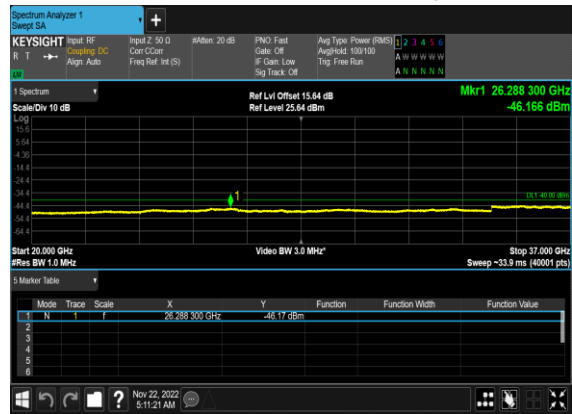
N48(10M)_DFT-s-OFDM_BPSK_Outer_Full_High_CH
