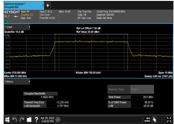
N26(5M)_DFT-s-OFDM_QPSK_Outer_Full_Mid_CH
