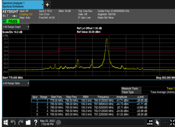
N14(5M)_DFT-s- OFDM_BPSK_Edge_1RB_Right_Low_CH
