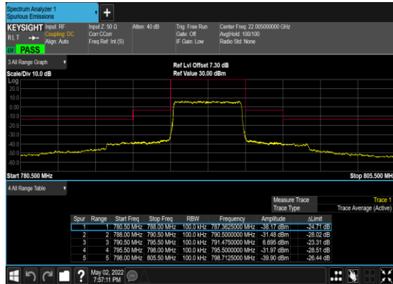
N14(5M)_DFT-s- OFDM_QPSK_Outer_Full_Mid_CH
