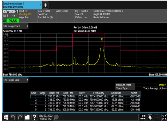
N14(5M)_DFT-s- OFDM_QPSK_Edge_1RB_Right_Mid_CH
