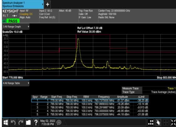
N14(5M)_DFT-s- OFDM_BPSK_Edge_1RB_Left_Low_CH
