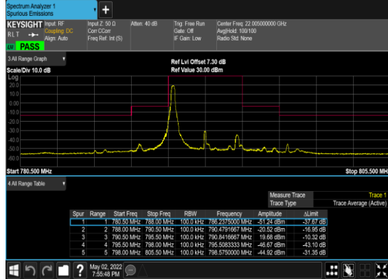
N14(5M)_DFT-s- OFDM_QPSK_Edge_1RB_Left_Mid_CH
