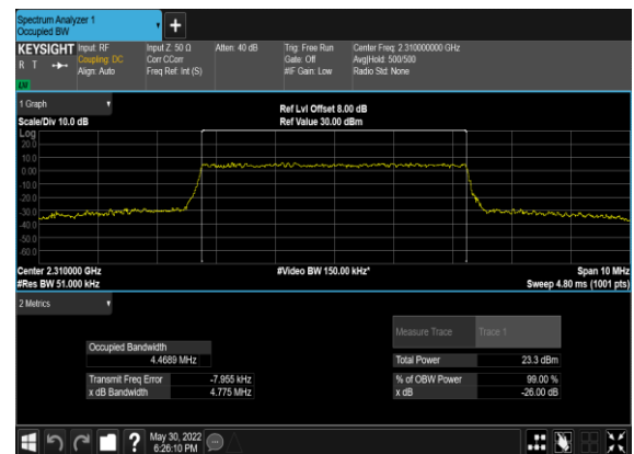
N30(5M)_CP-OFDM_256 QAM_Outer_Full_Mid_CH
