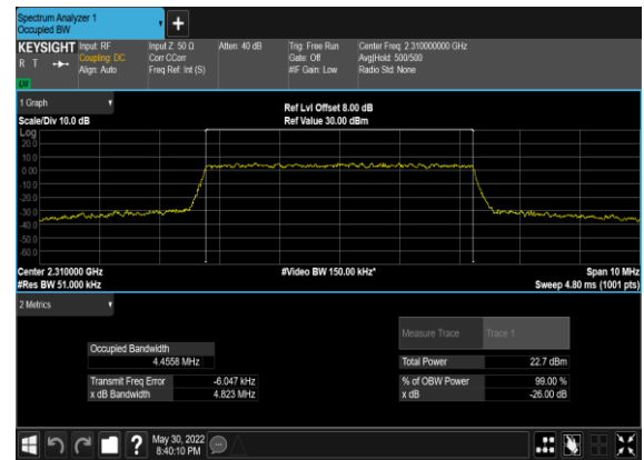
N30(5M)_CP-OFDM_16 QAM_Outer_Full_Mid_CH
