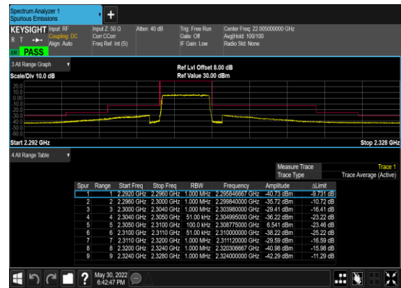
N30(5M)_DFT-s-OFDM_QPSK_Outer_Full_Low_CH
