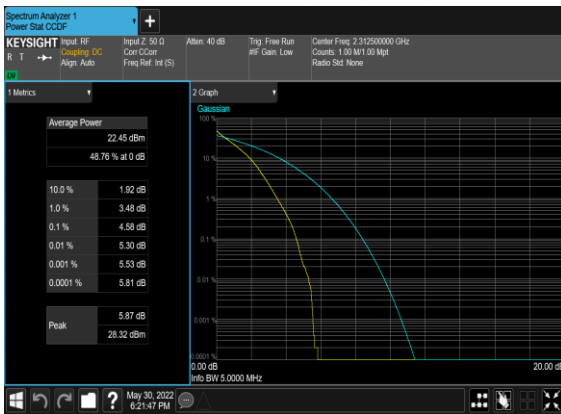
N30(5M)_DFT-s-OFDM_PI_2-BPSK_Outer_Full_High_CHN30(5M)_DFT-s-OFDM_PI_2-BPSK_Edge_1RB_Left_High_CH
