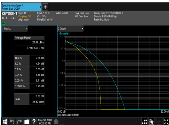
N30(5M)_DFT-s-OFDM_QPSK_Outer_Full_High_CH
