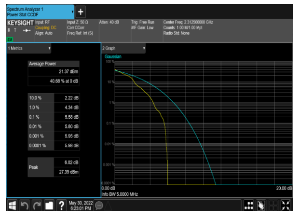
N30(5M)_DFT-s-OFDM_QPSK_Edge_1RB_Left_High_CH
