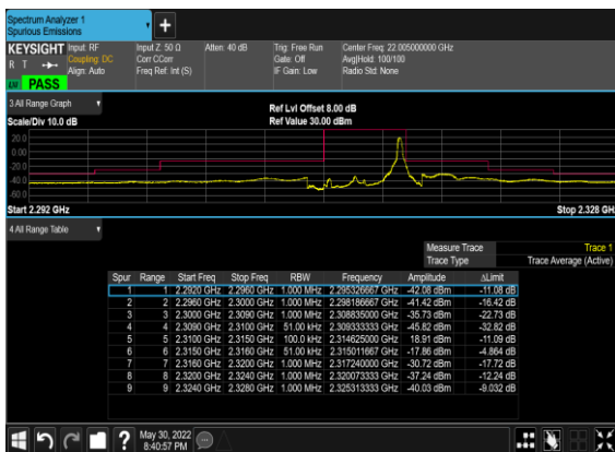
N30(5M)_DFT-s-OFDM_BPSK_Edge_1RB_Right_High_CH
