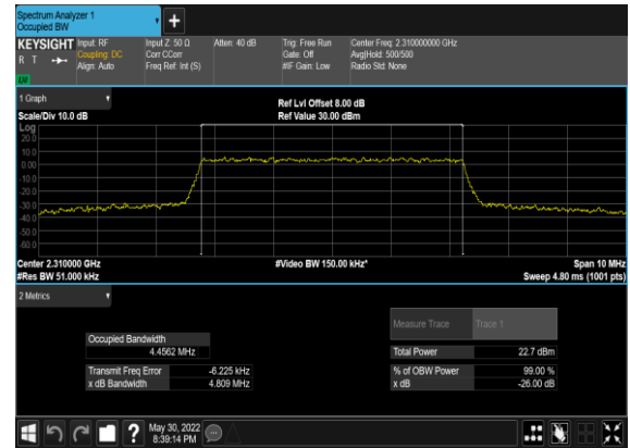
N30(5M)_DFT-s-OFDM_QPSK_Outer_Full_Mid_CH
