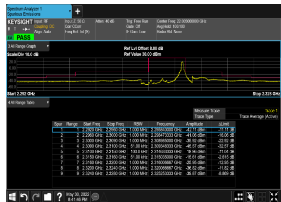
N30(5M)_DFT-s-OFDM_QPSK_Edge_1RB_Right_High_CH
