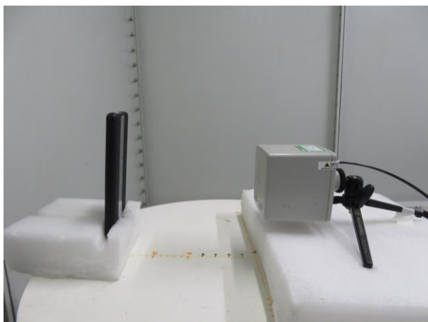
Position E, test separation 20cm
