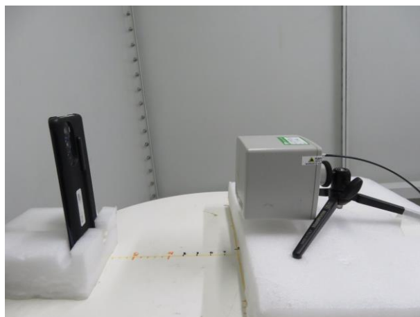
Position F, test separation 20cm
