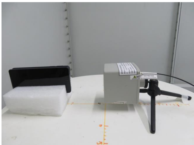
Position A, test separation 10cm
