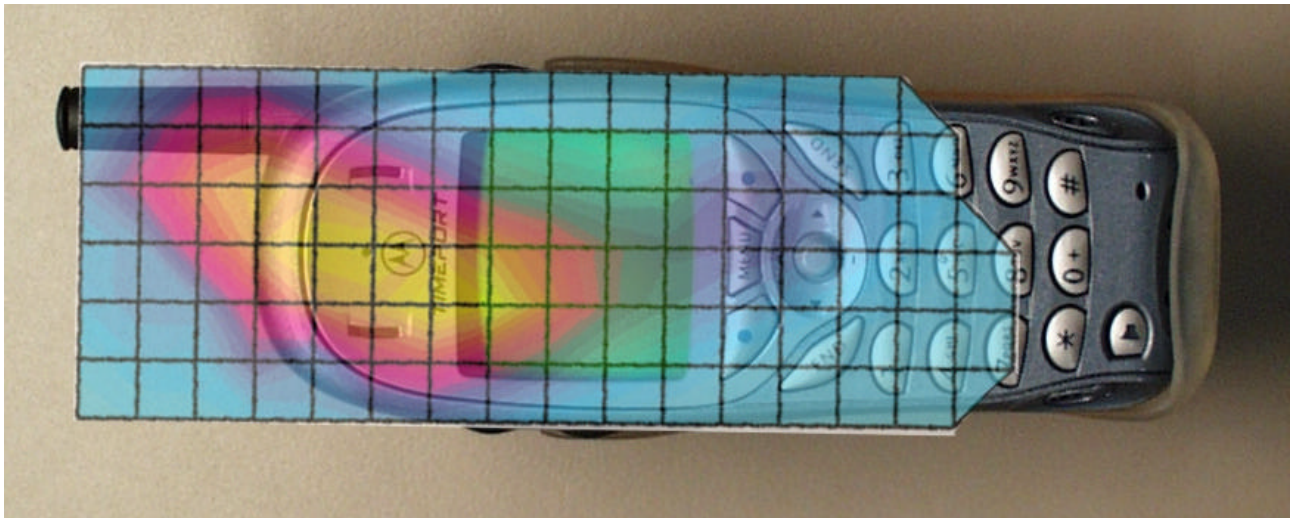
Figure 2. Front of Phone with typical 1900MHz Contour Plot Overlaid.
