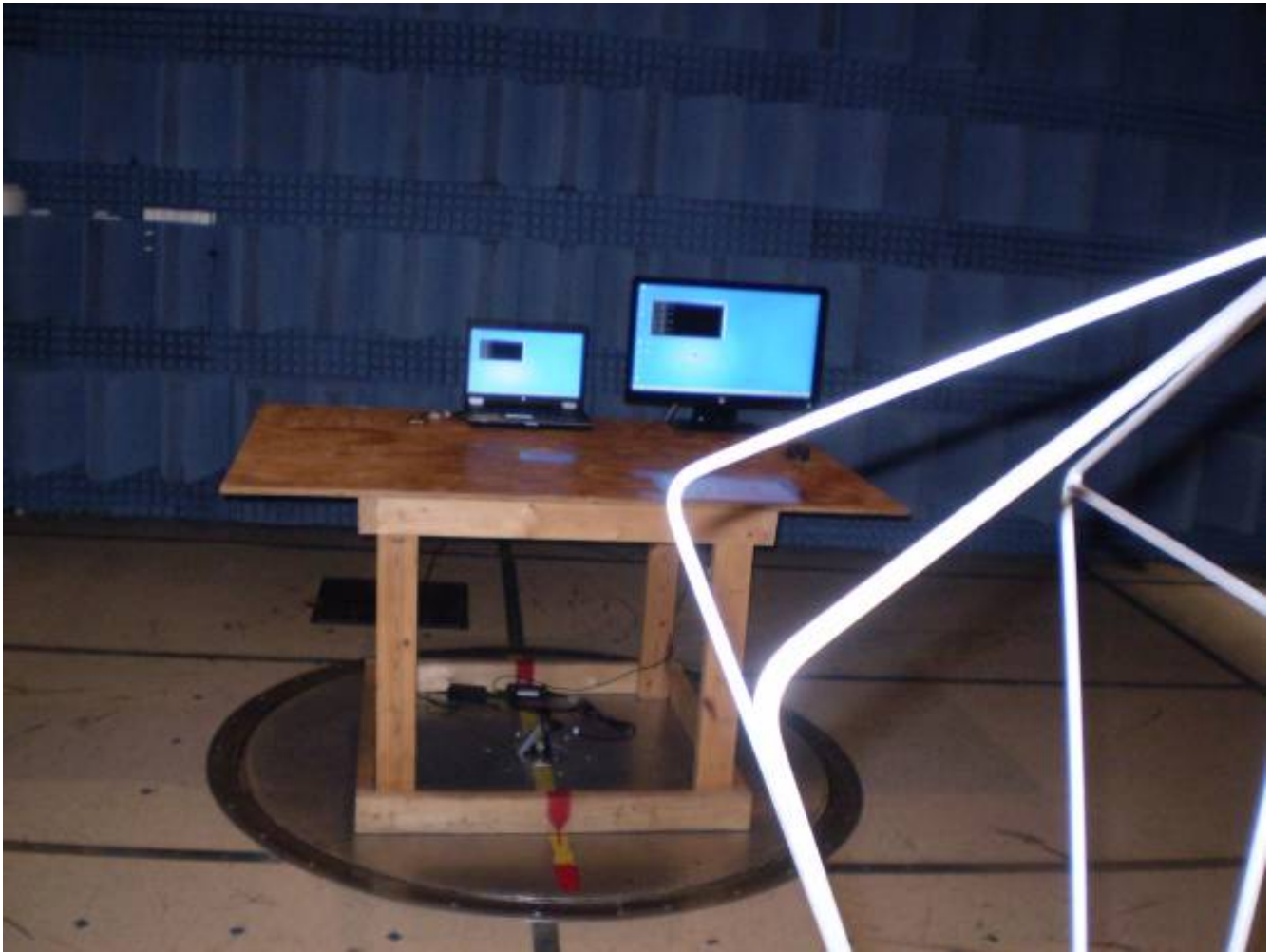
Figure 7c2-1: Spurious Radiations (Part 15 Computing Device).
