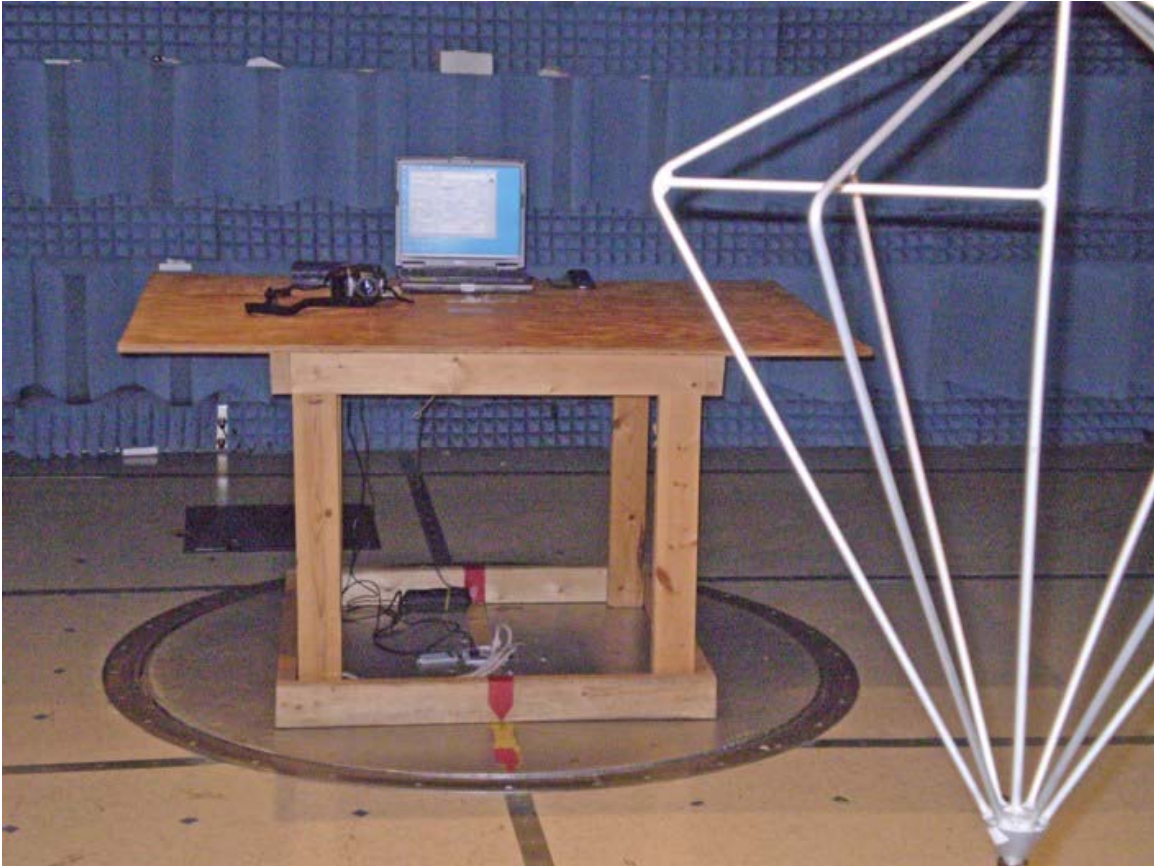
EMC Report #23308 Part 15, PC Peripheral
