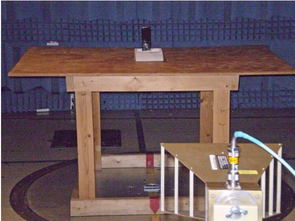
EMC Report #23308 Tx Radiated
